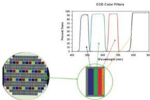
Figure 3. Example of a 4-color patterned filter deposited onto a 200 mm wafer. Each element,
