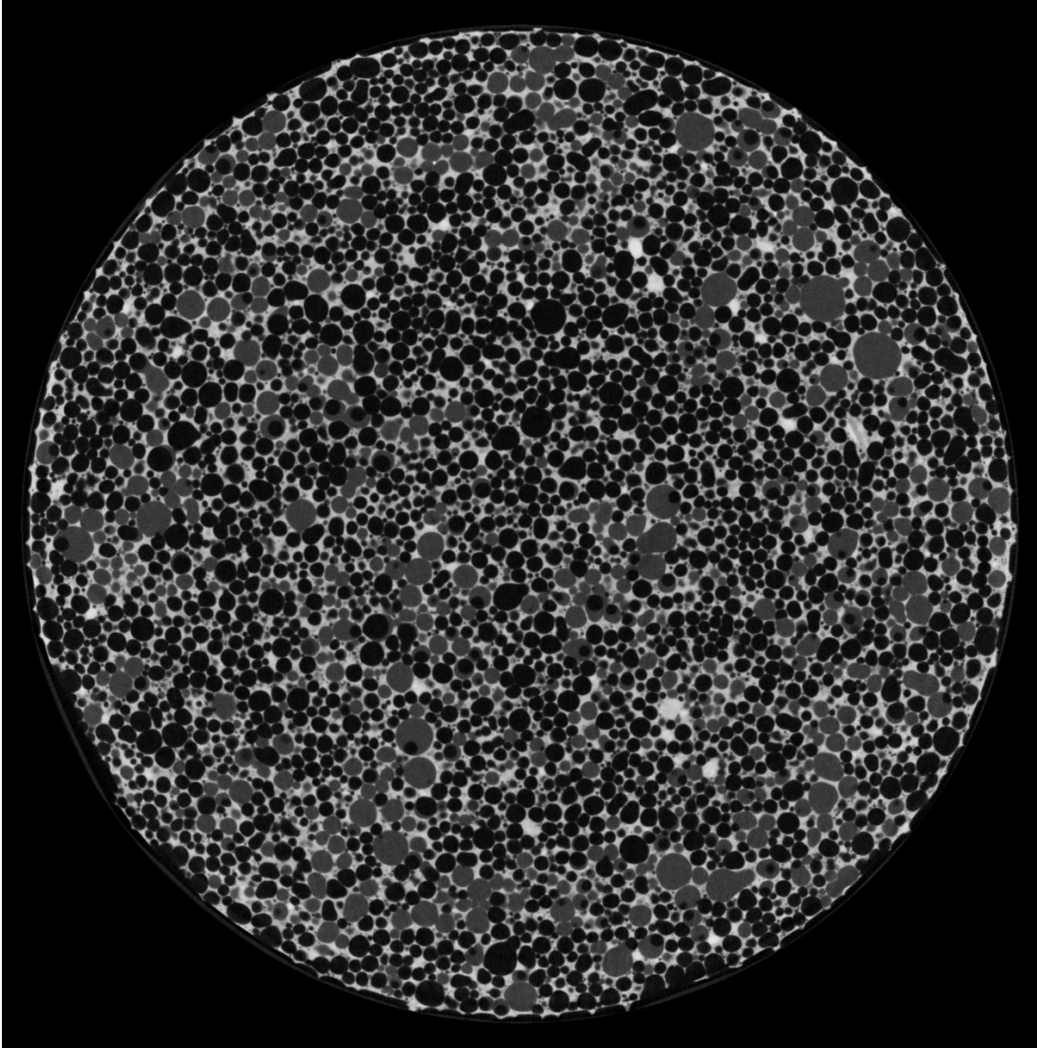
Figure 7-10 CT scan image of specimen B1-23 after the V8 treatment
