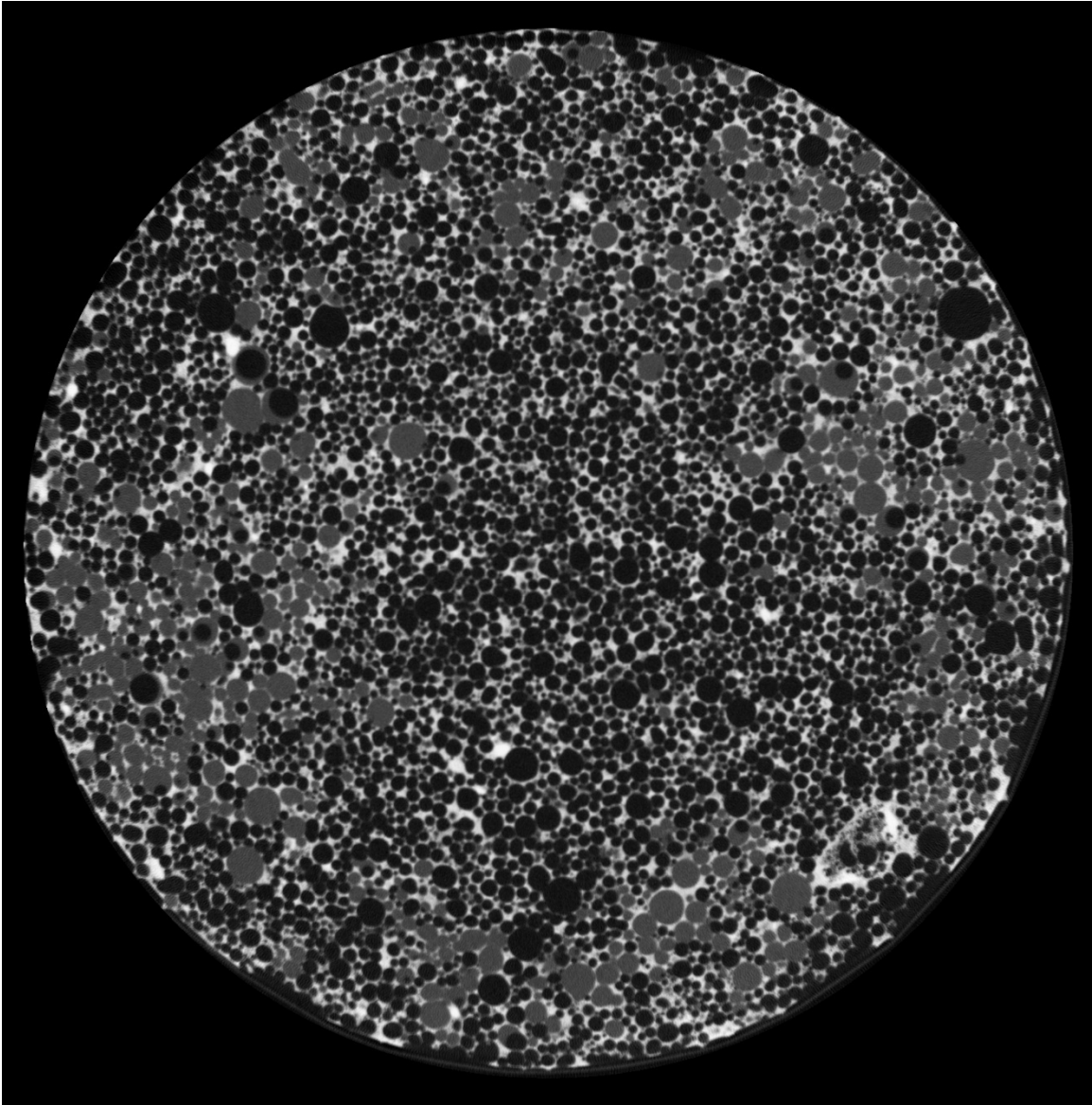
Figure 7-18 CT scan image of specimen B3-24 after the V8 treatment
