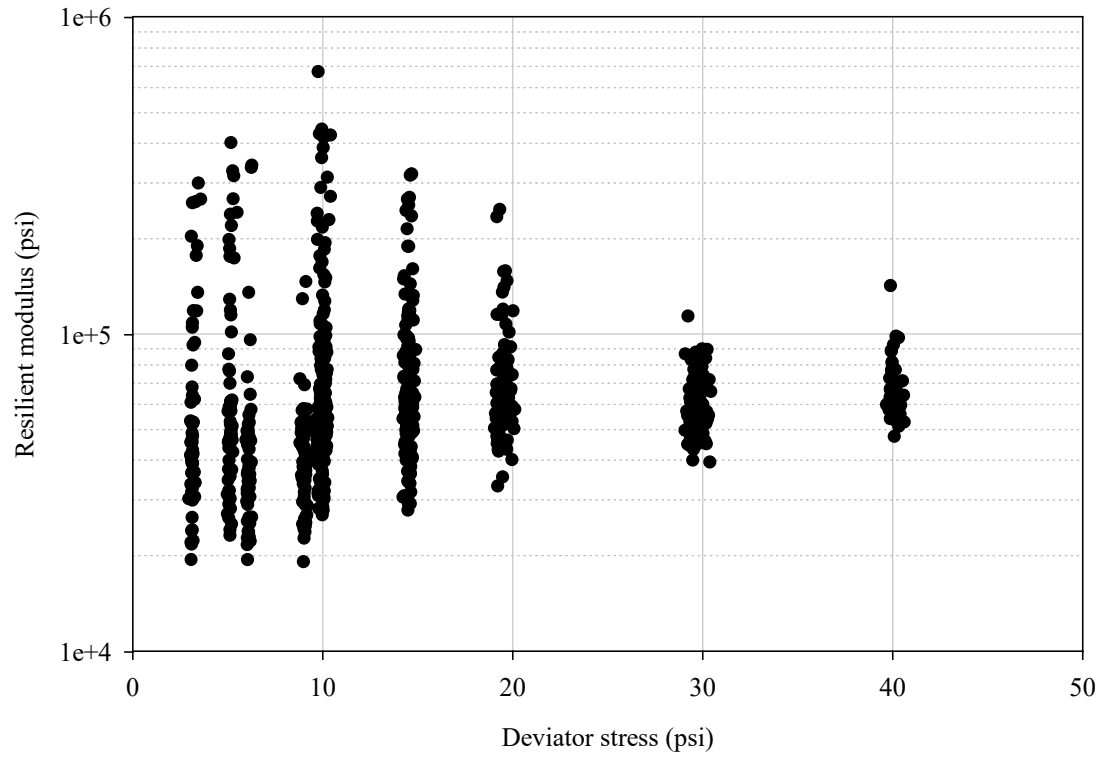
Figure 9-3 Resilient modulus of the LCC specimens as a function of the applied deviator stress
