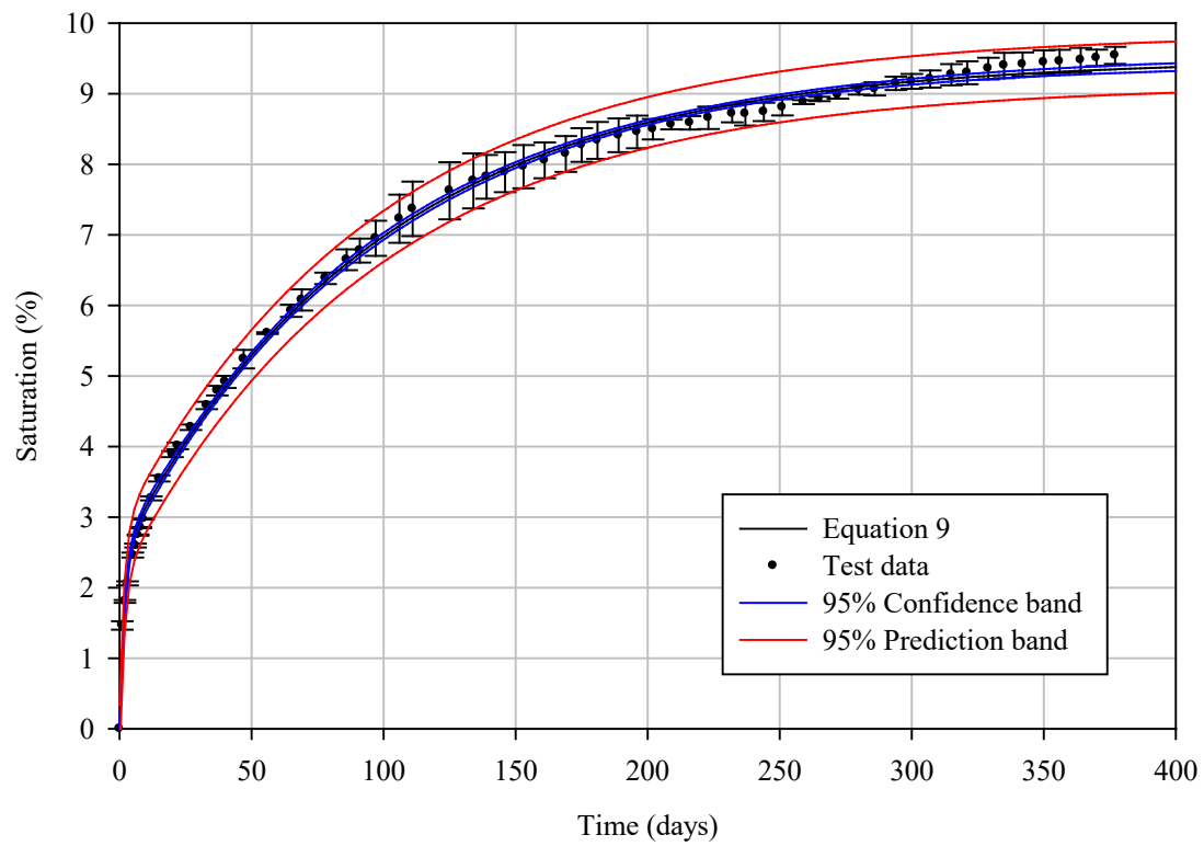
Figure 7-6 Long-term degree of saturation regression model (Equation 7-1) for B3-30, B3-31, and B3-32 with confidence and prediction bands
