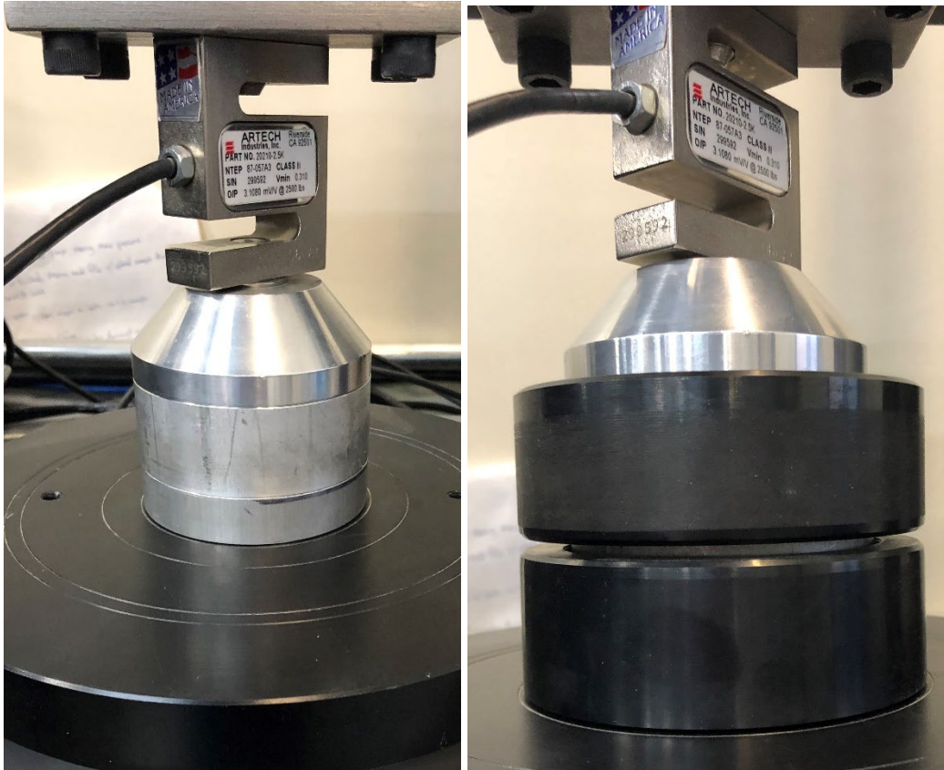
Figure 10-1 Photo of the 7075-aluminum system compliance calibration disc
