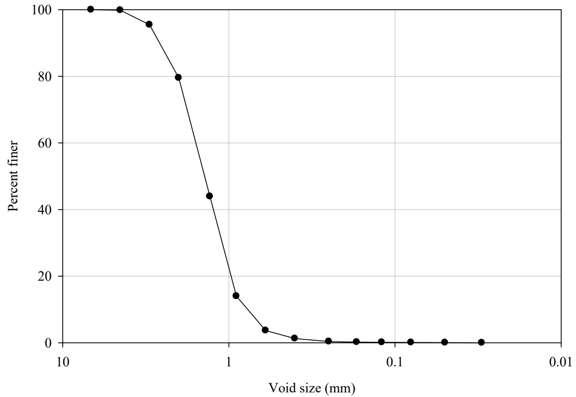
Figure 6-12 Combined VSD estimations for all WipFrag analyses
