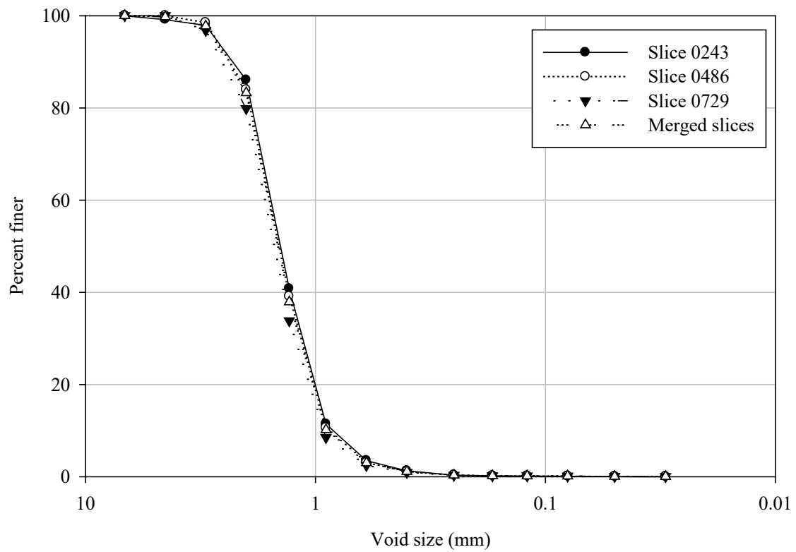
Figure 6-8 VSD estimations for Sample B1-23
