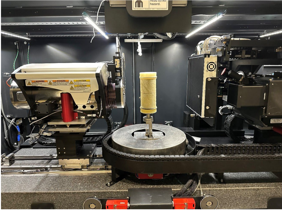
Figure 6-4 Photograph of a test specimen prepared for CT scanning
