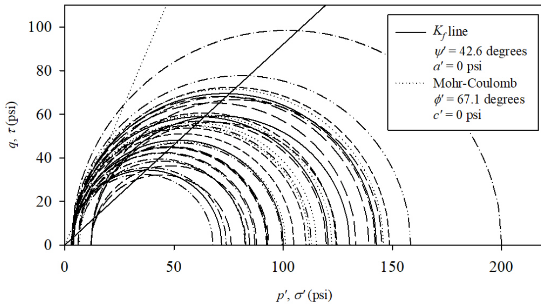
Figure 11-8 Mohr's circles, K_f line, and Mohr-Coulomb failure envelope for the peak stress points for all triaxial tests
