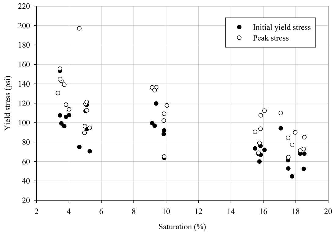
Figure 11-6 Yield stresses in triaxial compression of the LCC specimens as a function of saturation
