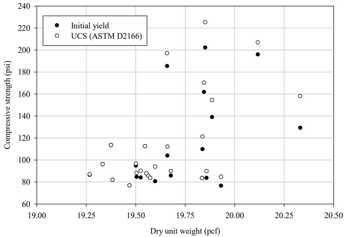
Figure 10-5 Initial yield and the UCS of the cured LCC specimens as a function dry unit weight
