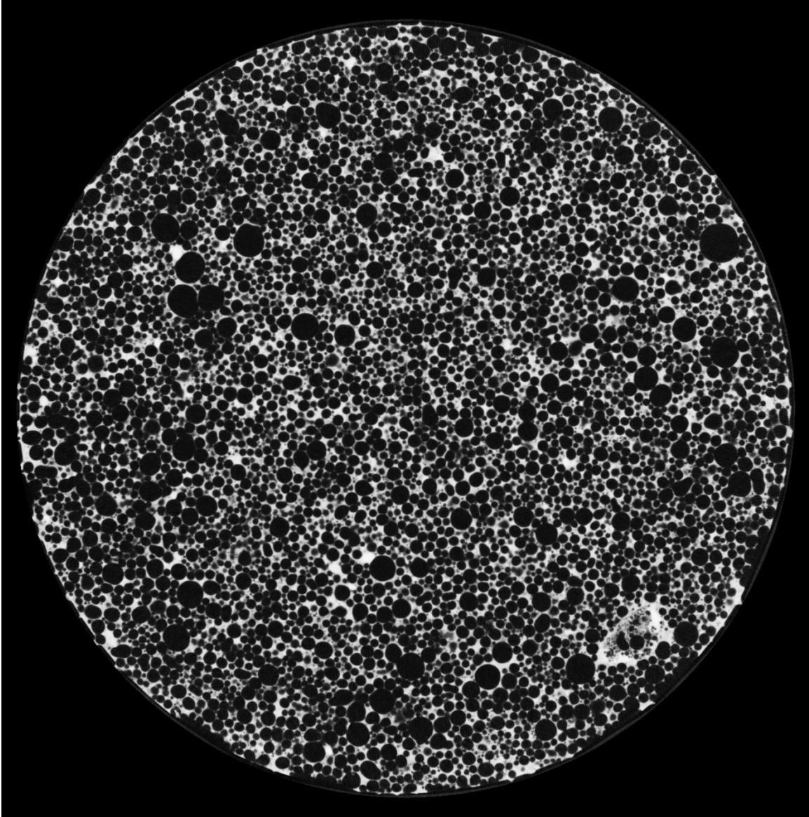
Figure 7-16 CT scan image of specimen B3-24 after the M5 treatment
