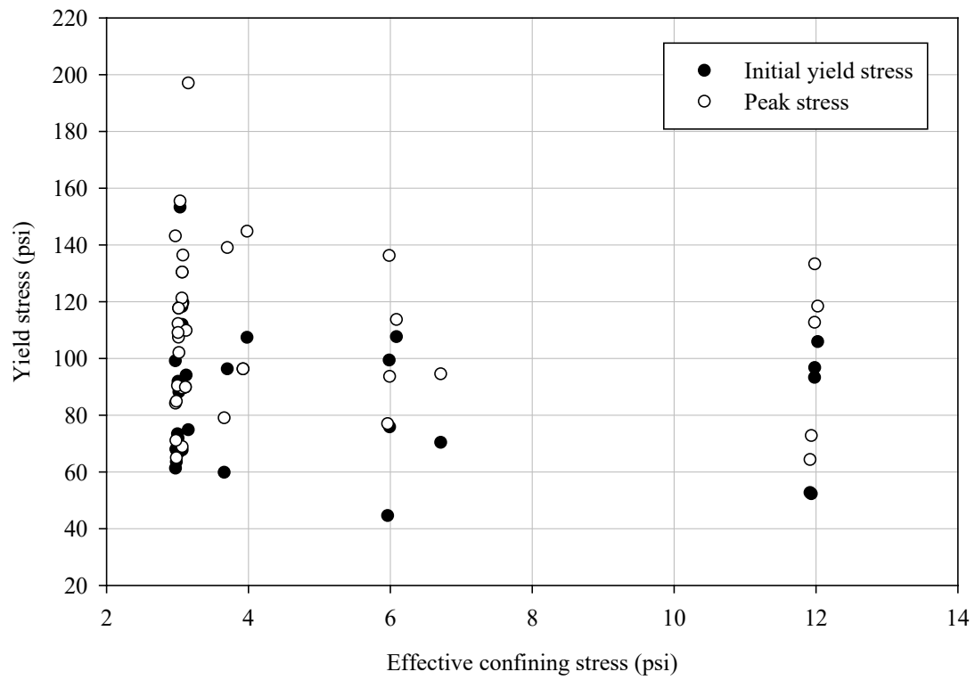
Figure 11-5 Yield stresses in triaxial compression of the LCC specimens as a function of the effective confining stress
