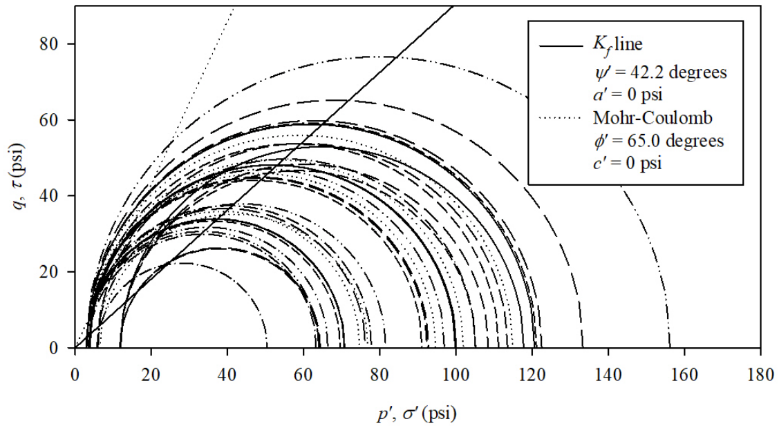
Figure 11-7 Mohr's circles, K_f line, and Mohr-Coulomb failure envelope for the initial yield points for all triaxial tests
