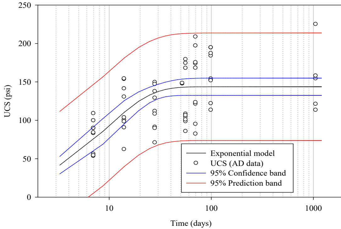
Figure 10-9 Unconfined compressive strength as a function of curing time and the regression model (Equation 10-1) with confidence and prediction bands
