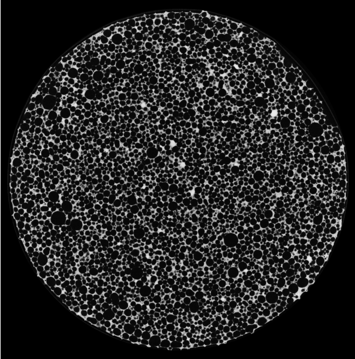
Figure 7-12 CT scan image of specimen B1-24 after the M5 treatment
