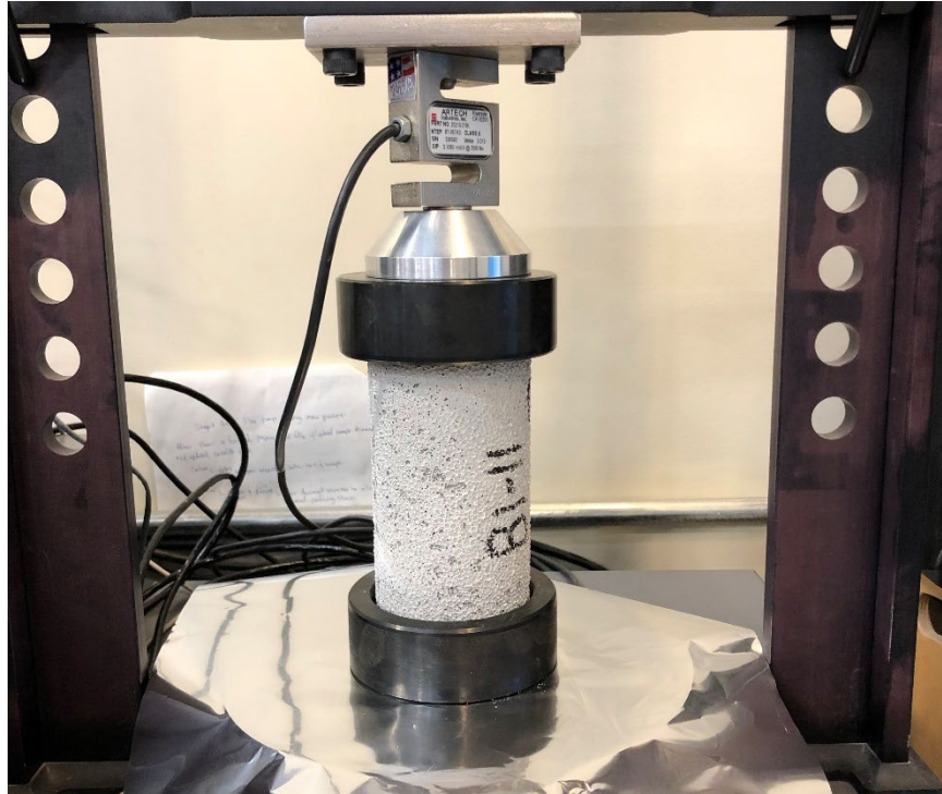
Figure 10-3 Photo of a specimen prepared for UCS testing in the load frame with padded end caps
