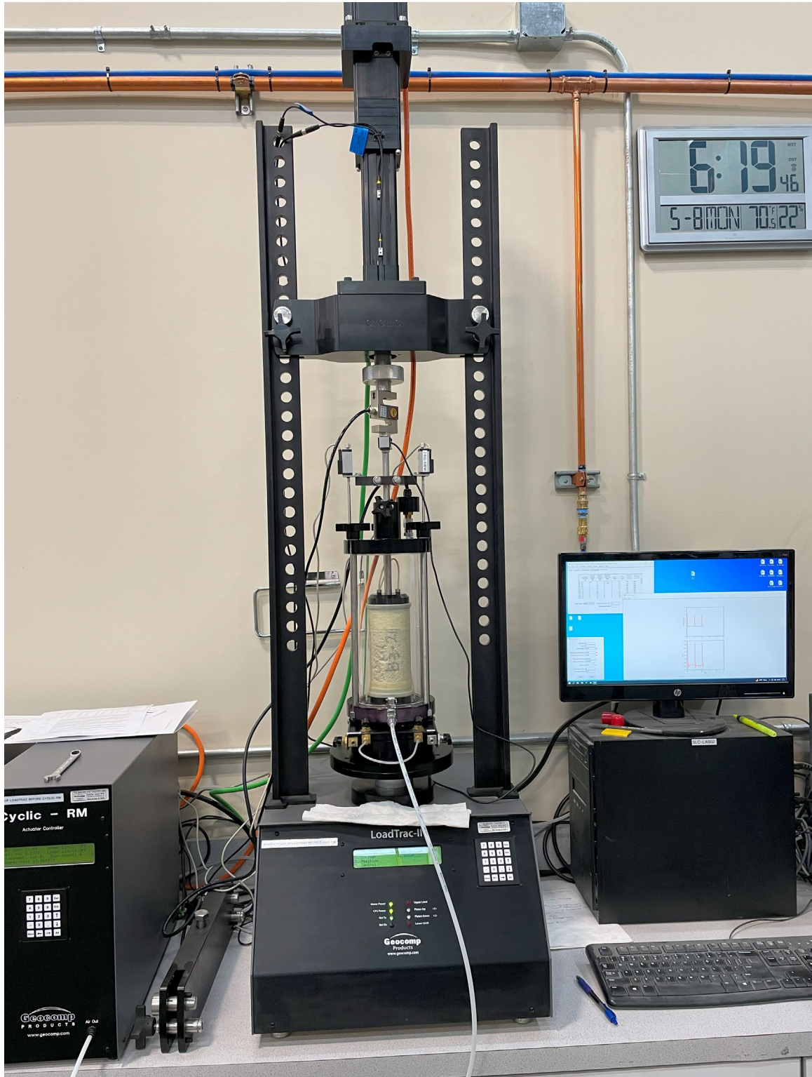
Figure 9-1 Photo of the resilient modulus testing apparatus
