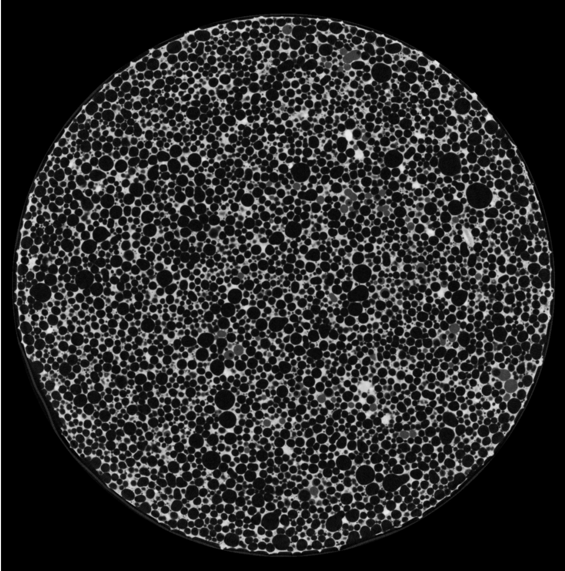
Figure 7-9 CT scan image of specimen B1-23 after the D1 treatment
