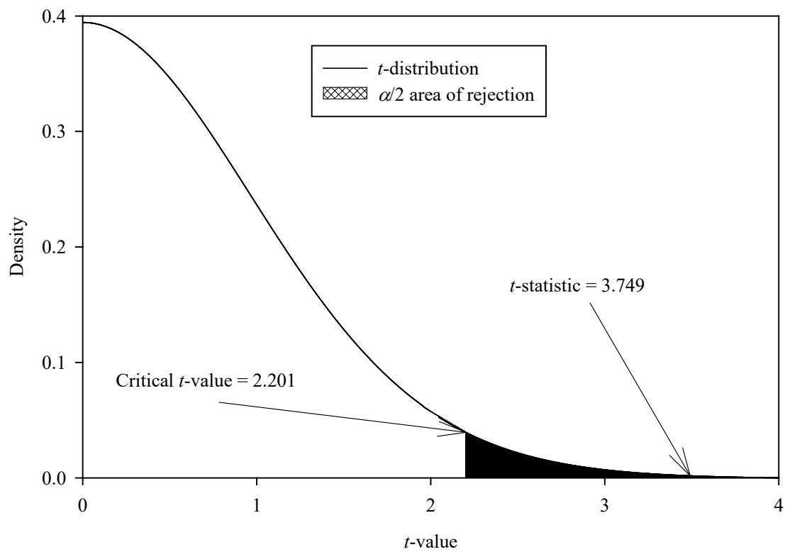
Figure 7-3 The t -distribution with the t -statistic and critical t -value identified
