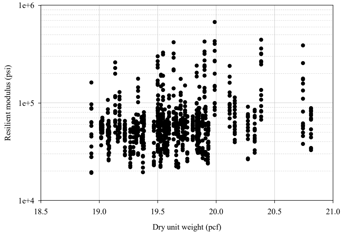
Figure 9-4 Resilient modulus of the LCC specimens as a function of the dry unit weight
