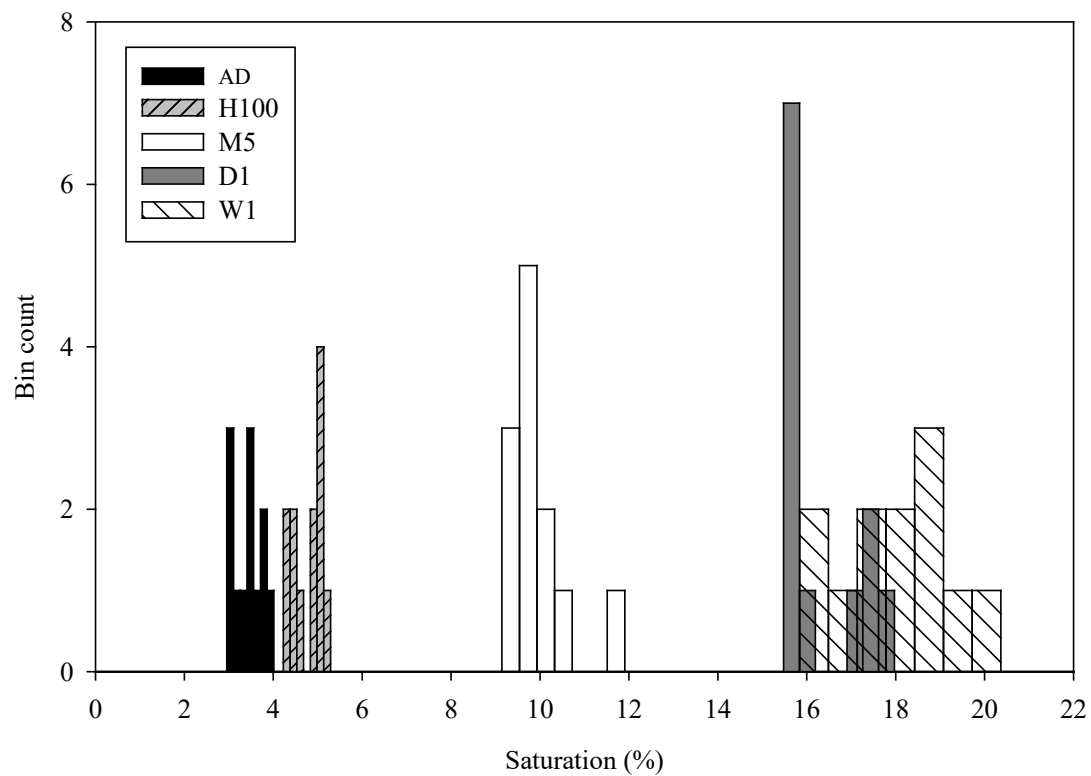
Figure 7-1 Histograms of the degrees of saturation resulting from each of the treatments
