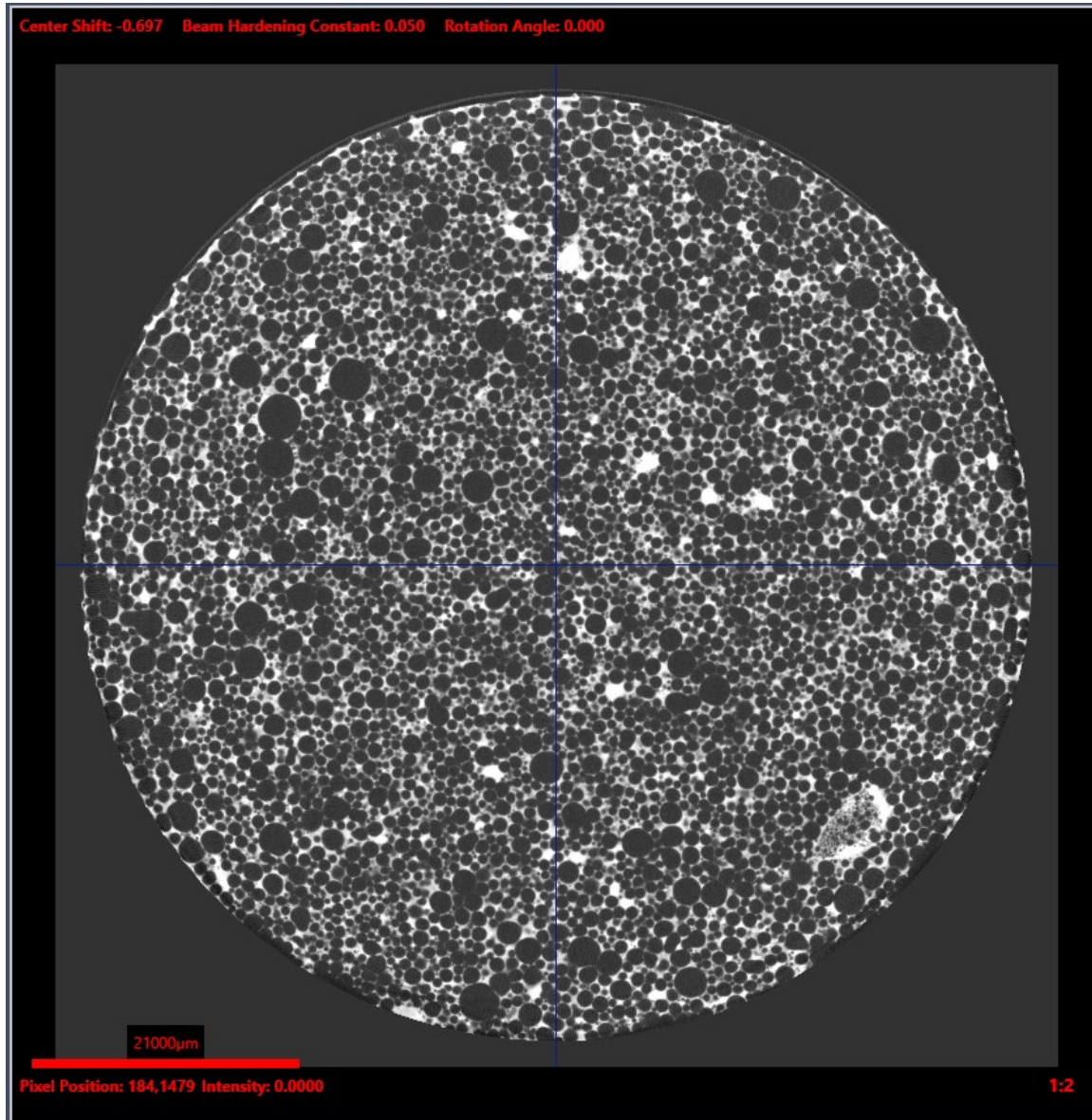
Figure 6-7 Initial view from the CT scan image reduction for sample B3-24
