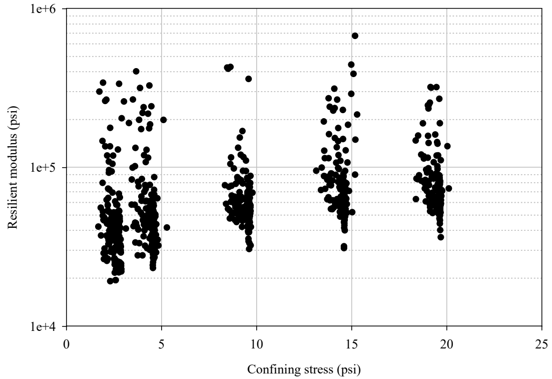
Figure 9-2 Resilient modulus of the LCC specimens as a function of confining stress
