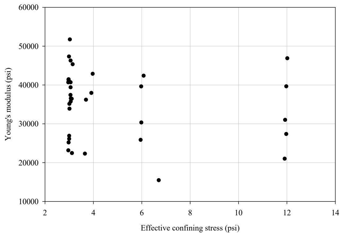
Figure 11-3 Triaxial Young's modulus of the LCC specimens as a function of the effective confining stress
