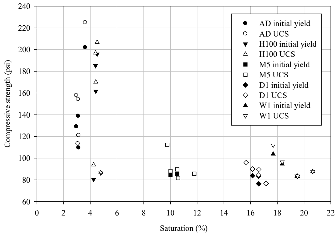
Figure 10-6 Initial yield and the UCS of the LCC specimens as a function of saturation
