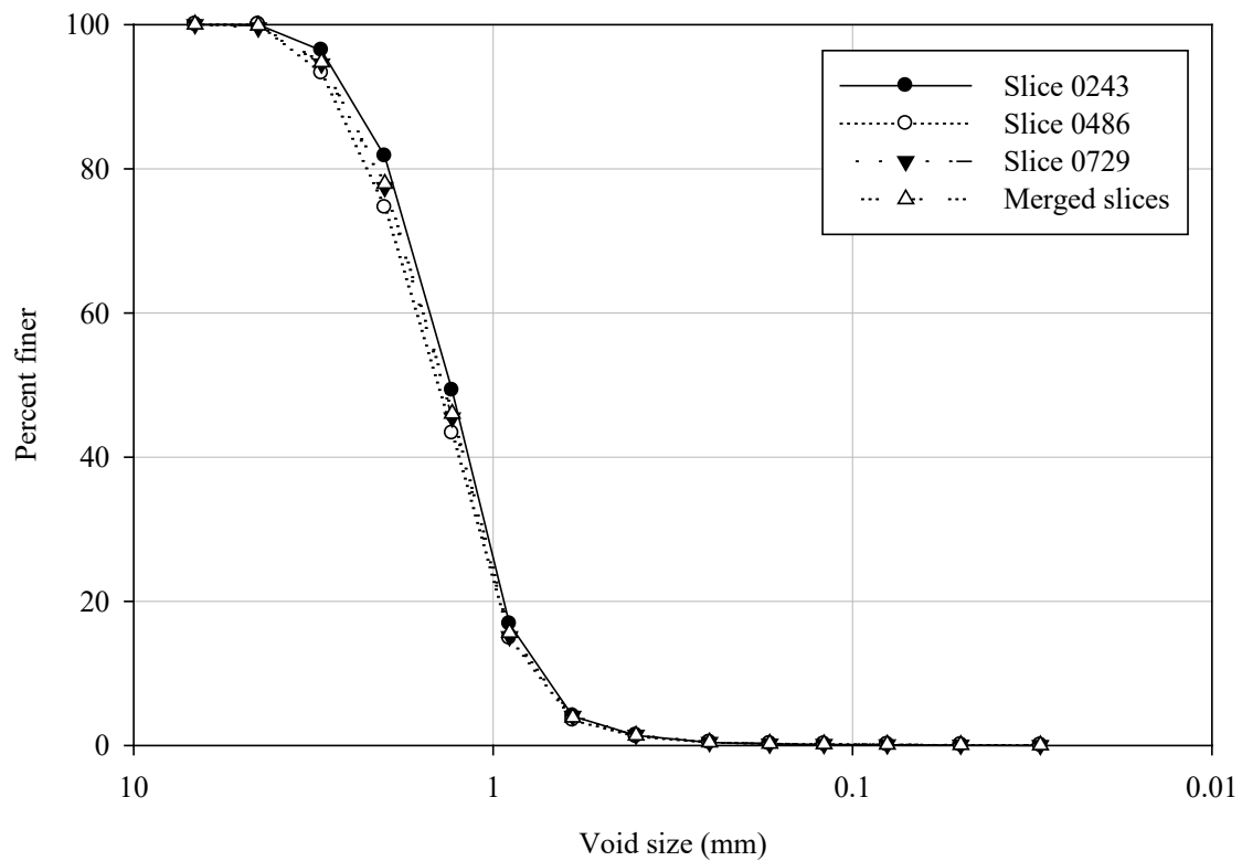
Figure 6-10 VSD estimations for Sample B3-24
