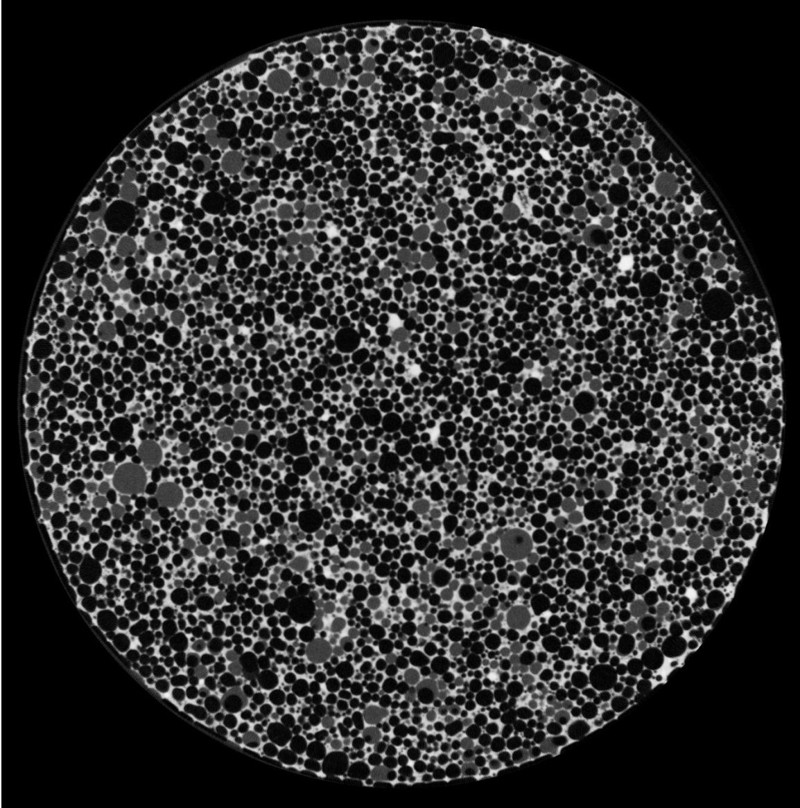
Figure 7-14 CT scan image of specimen B1-24 after the V8 treatment
