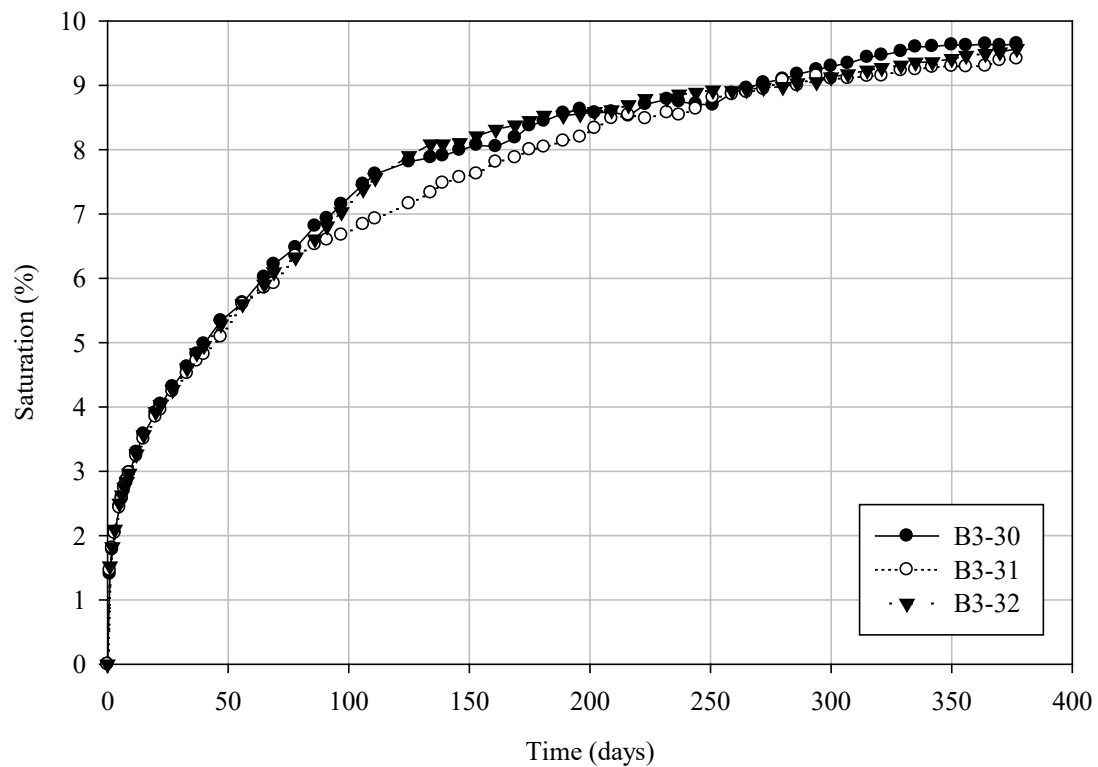
Figure 7-4 Saturation data as a function of time from the long-term saturation test
