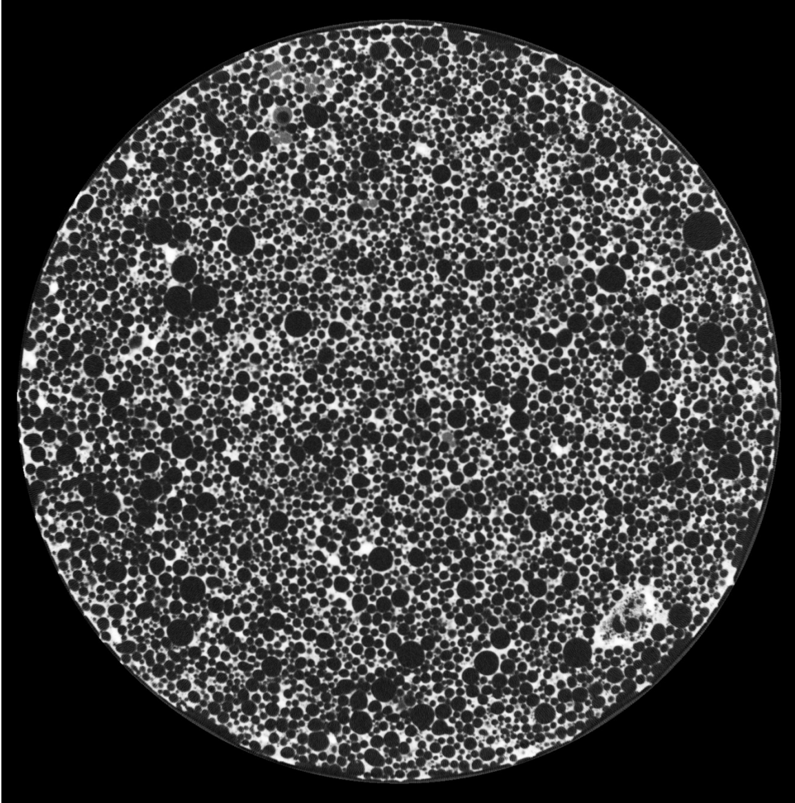
Figure 7-17 CT scan image of specimen B3-24 after the D1 treatment
