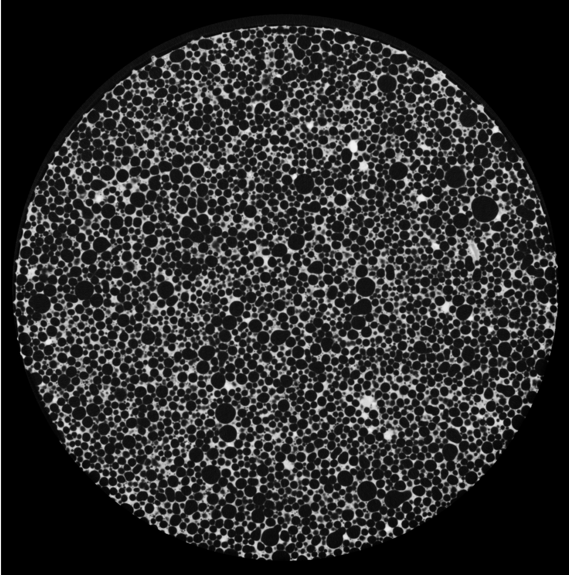
Figure 7-7 CT scan image of specimen B1-23 after the AD treatment
