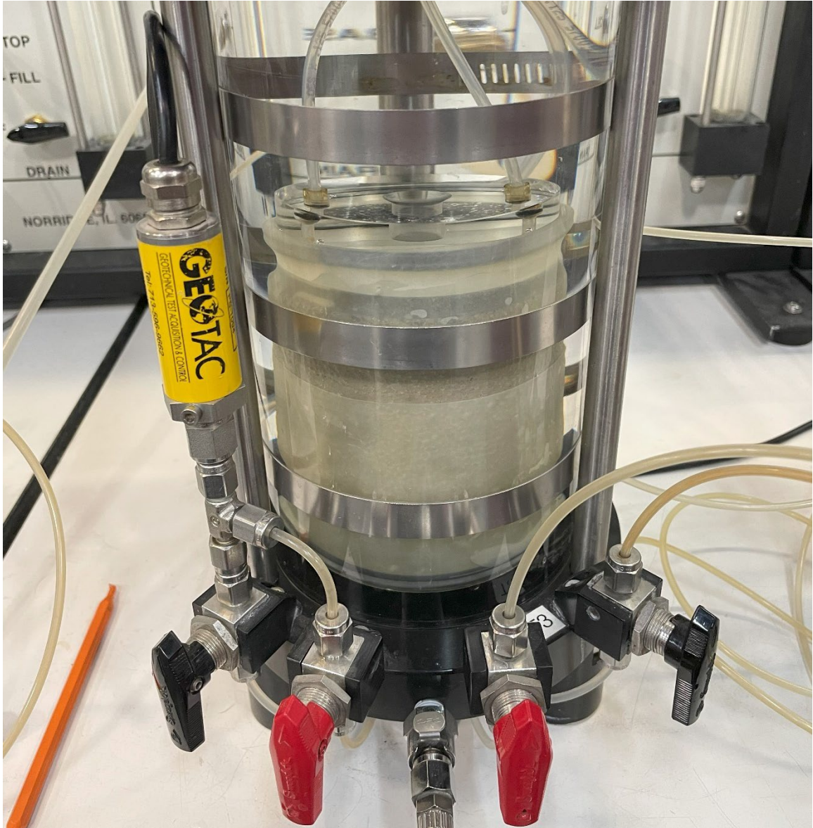
Figure 8-2 Photo of an LCC specimen in the hydraulic conductivity test cell
