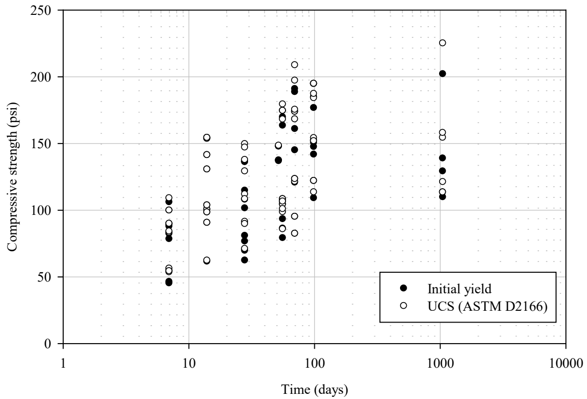
Figure 10-4 Initial yield and the UCS of the air-dried LCC specimens as a function of time
