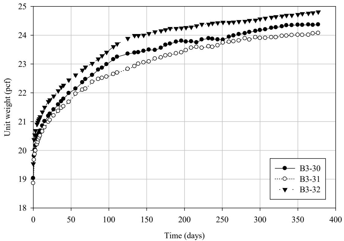
Figure 7-5 Total unit weight data as a function of time from the long-term saturation test
