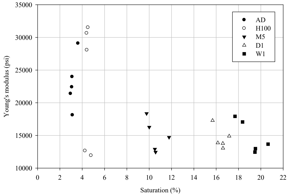
Figure 10-8 Young's modulus of the LCC specimens as a function of saturation
