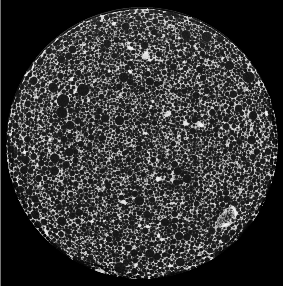
Figure 7-15 CT scan image of specimen B3-24 after the AD treatment
