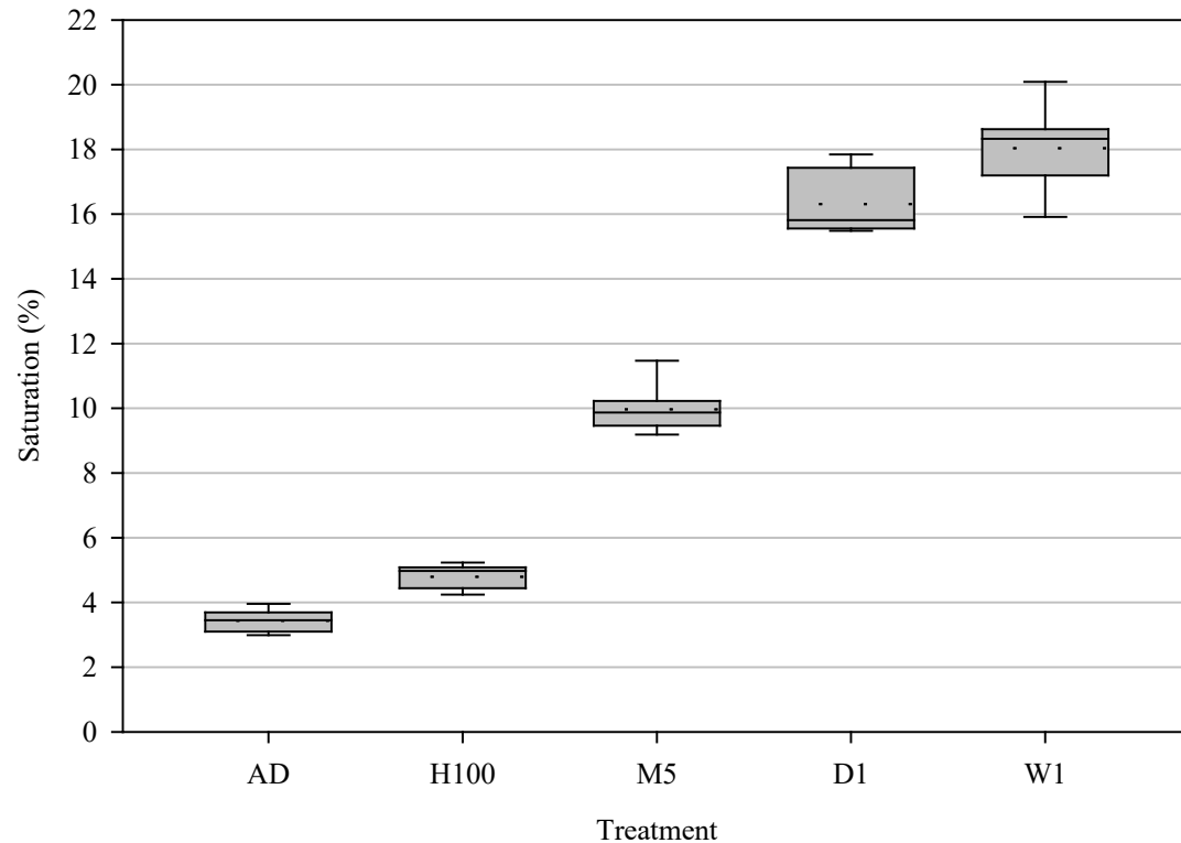
Figure 7-2 Box plot of the degrees of saturation resulting from each of the treatments
