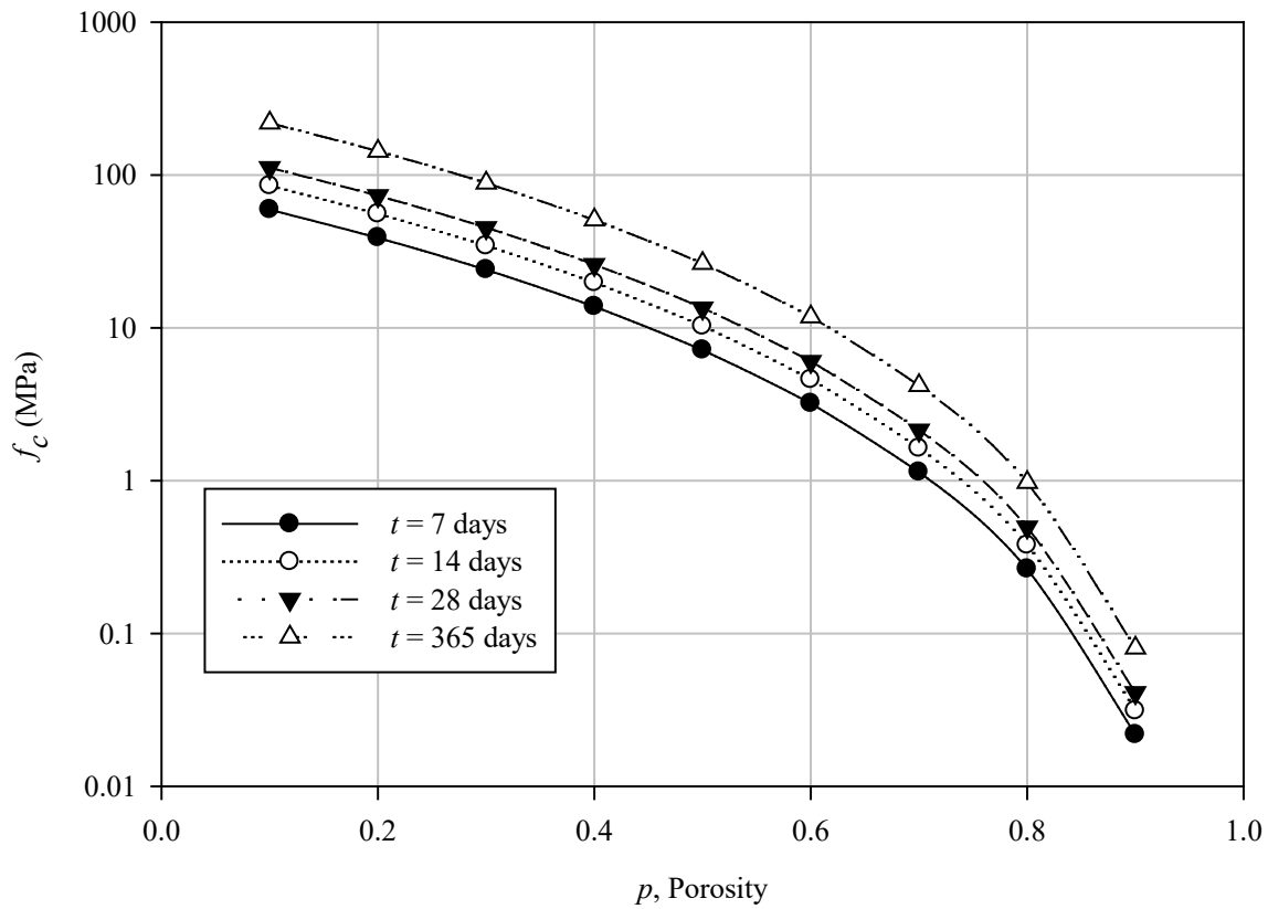
Figure 5-1 Estimated unconfined compressive strength as a function of porosity and time
