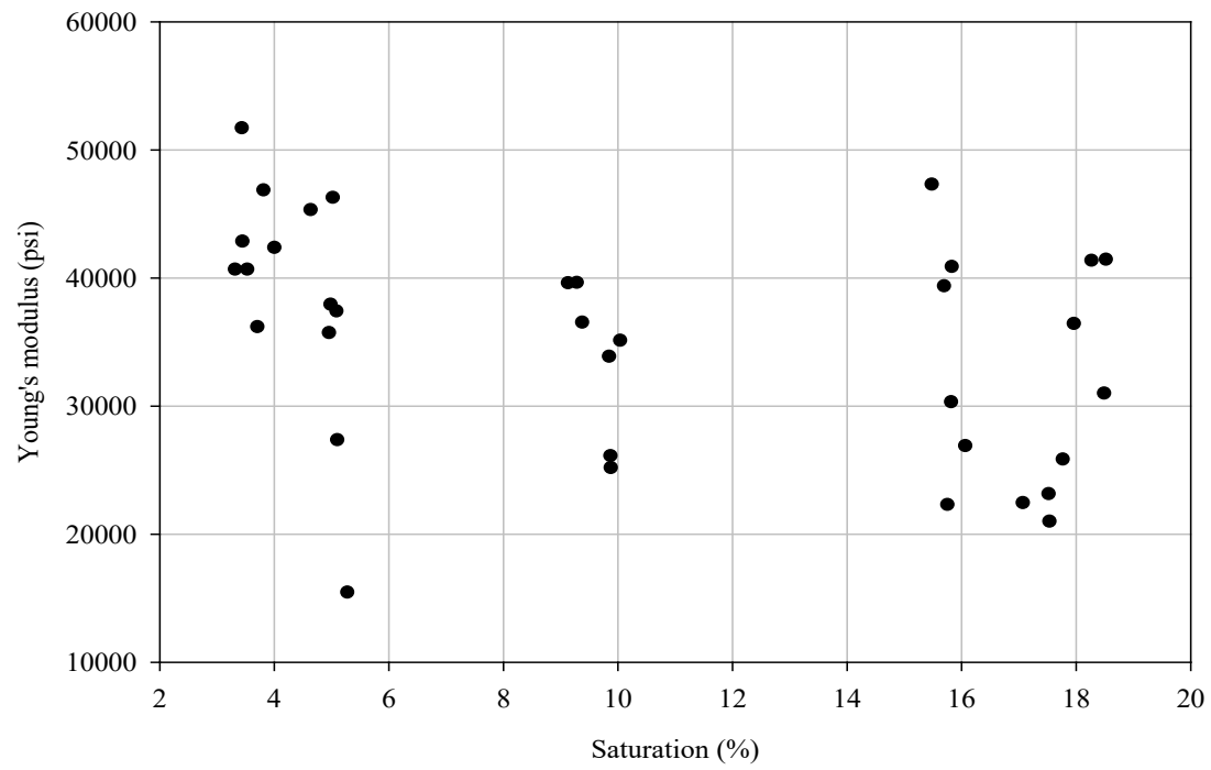
Figure 11-2 Triaxial Young's modulus of the LCC specimens as a function of saturation
