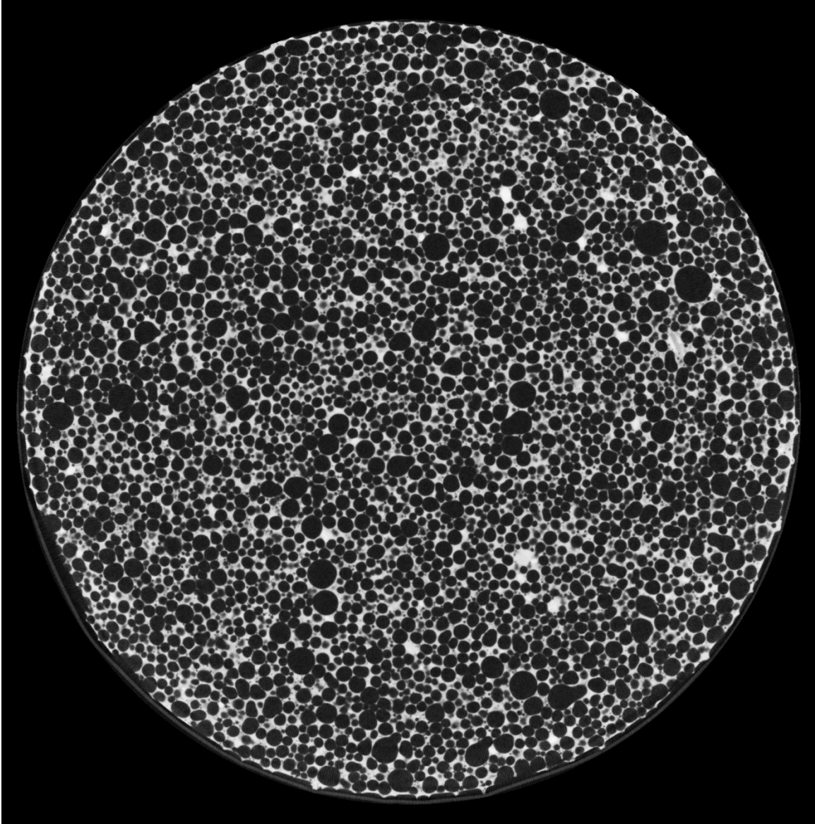
Figure 7-8 CT scan image of specimen B1-23 after the M5 treatment
