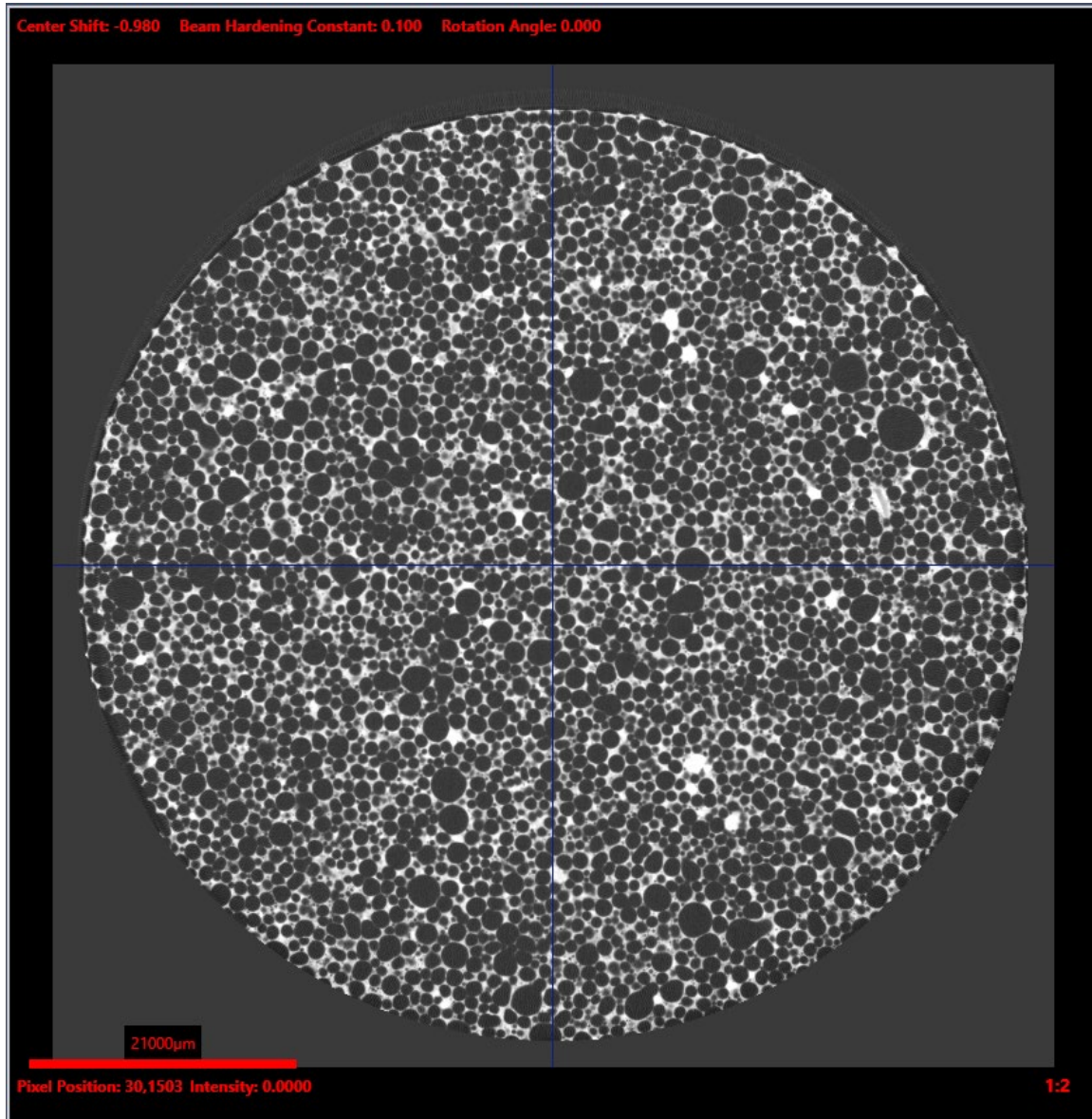
Figure 6-5 Initial view from the CT scan image reduction for sample B1-23
