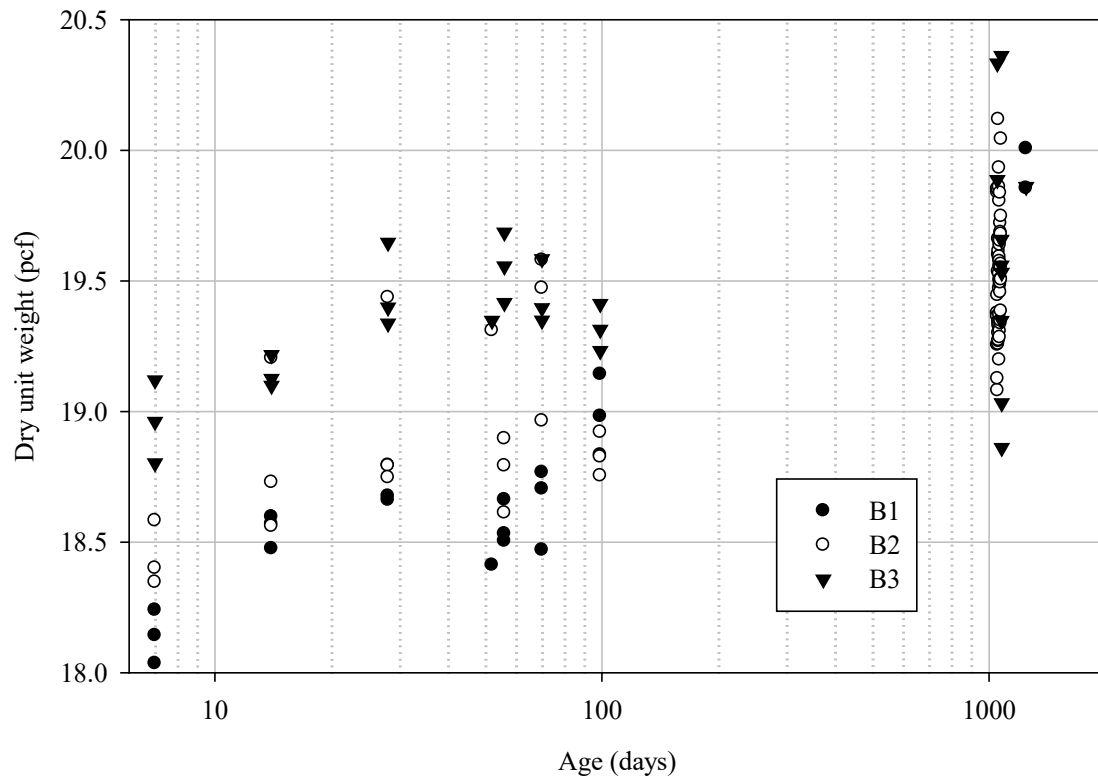
Figure 6-2 Dry unit weight for the LCC specimens as a function of time
