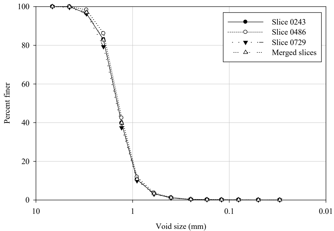
Figure 6-9 VSD estimations for Sample B1-24
