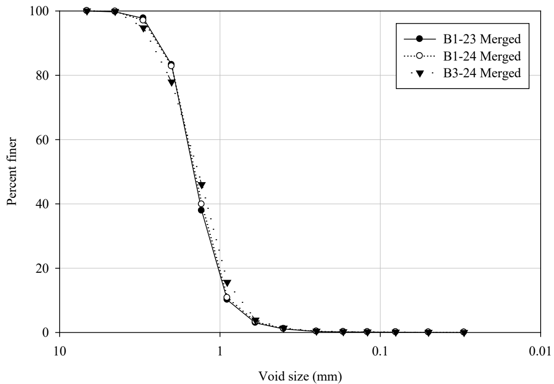
Figure 6-11 Merged respective VSD estimations for Samples B1-23, B1-24, and B3-24
