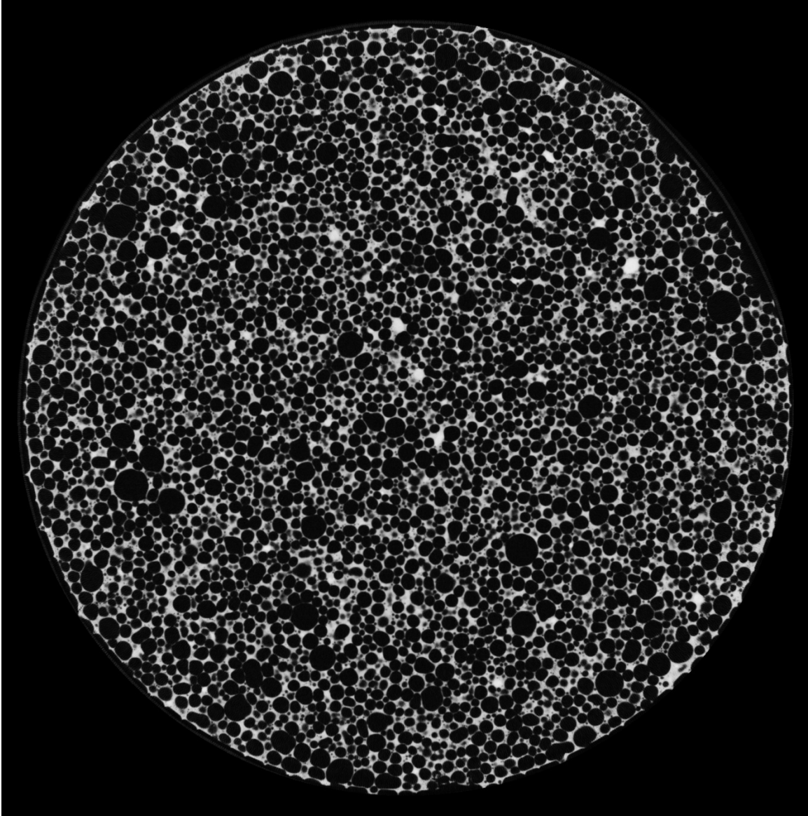
Figure 7-13 CT scan image of specimen B1-24 after the D1 treatment
