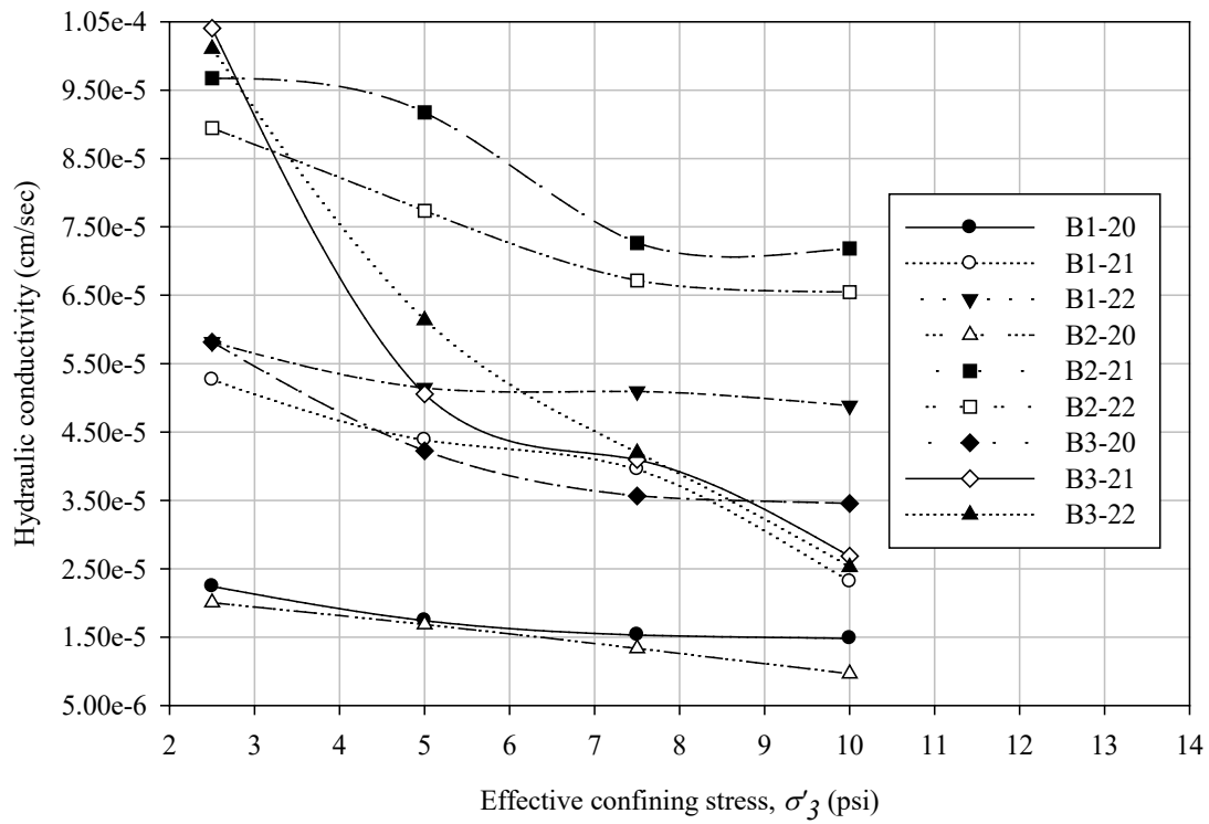
Figure 8-3 Hydraulic conductivity over a range of effective confining stresses
