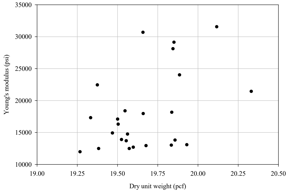
Figure 10-7 Young's modulus of the LCC specimens as a function of dry unit weight
