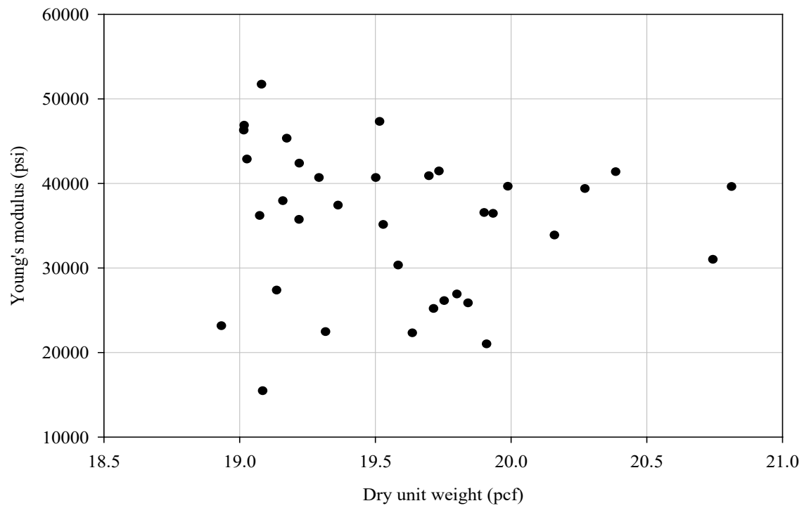
Figure 11-4 Triaxial Young's modulus of the LCC specimens as a function of the dry unit weight.
