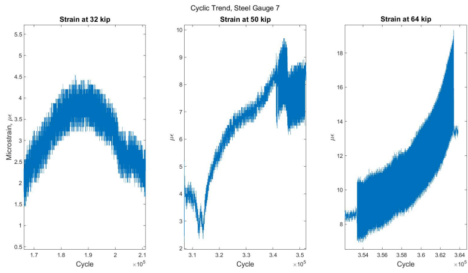
Figure F.22 Steel Gauge 7 – Cyclic Trend
