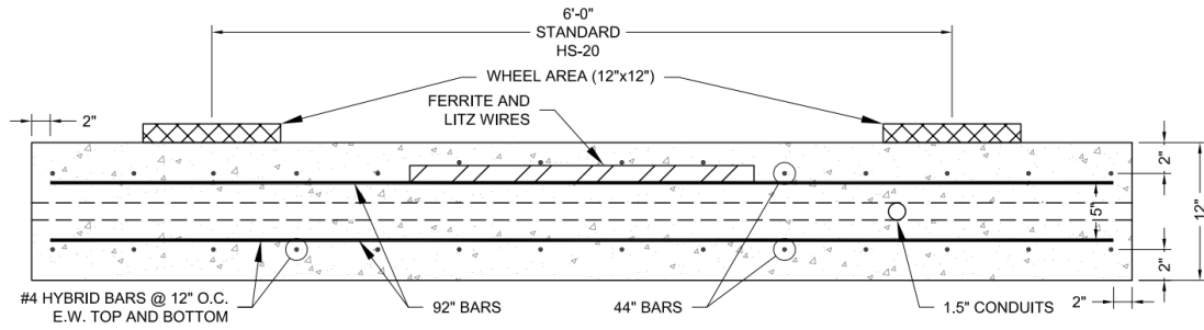
Figure 3.1 Cross-Section of System
