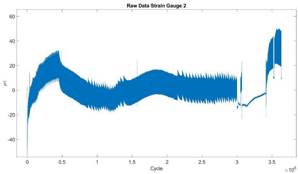
Figure F.5 Steel Gauge 2. Raw
