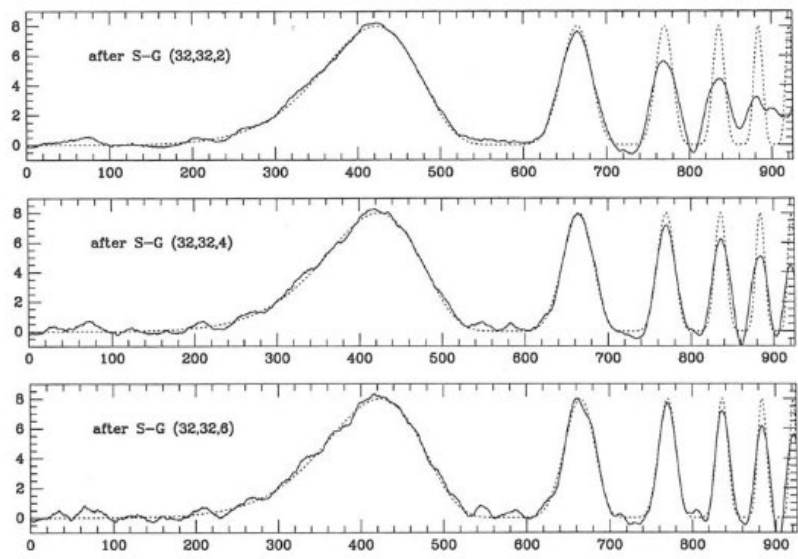
Figure 2.2 Example of an S-G Filter
