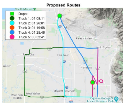
Figure 5.5 Proposed plowing routes for Paint (animation: https://youtu.be/rhCsKgMmJ2w )
