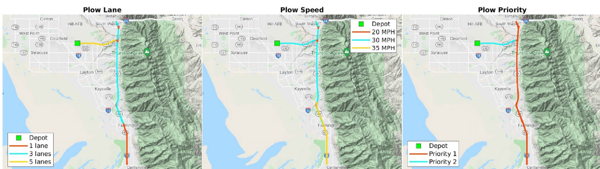
Figure 3.9 Plowing lanes, travel speed and road priorities along US-89 in group 2 within Clearfield
