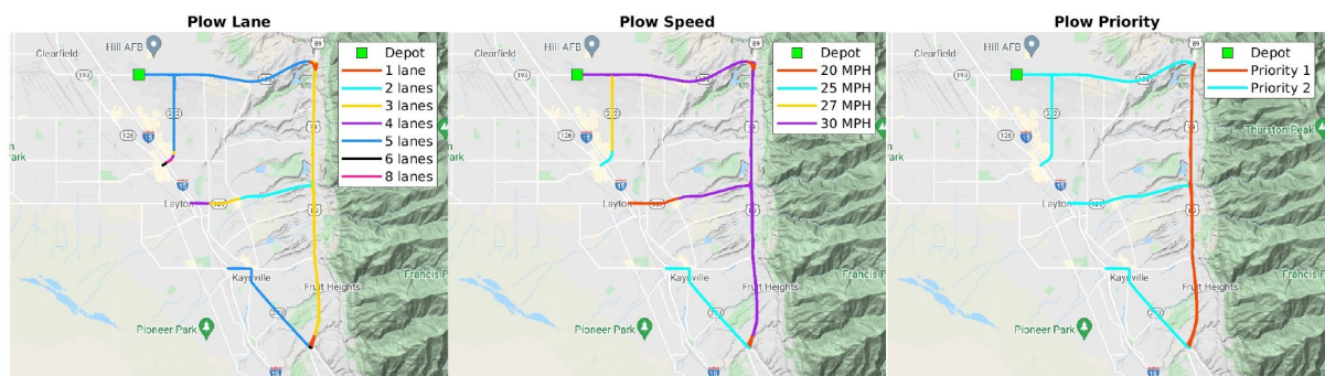
Figure 3.11 Plowing lanes, travel speed and road priorities along SR-109, SR-232 and SR-273 in group 4 within Clearfield
