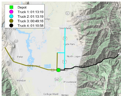
Figure 3.52 Proposed two-truck echelon routes along US-91 within south Logan (animation: https://youtu.be/_ZGcAd7yxRA )
