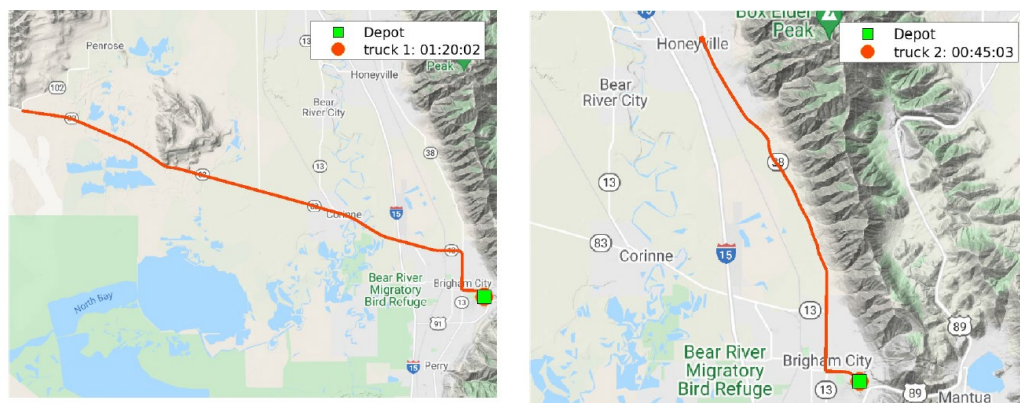
Figure 3.3 UDOT plowing routes along SR-83 and SR-38 (animation: https://youtu.be/a3dRAPnQKbU ; https://youtu.be/kFUTUyMdeeY )
