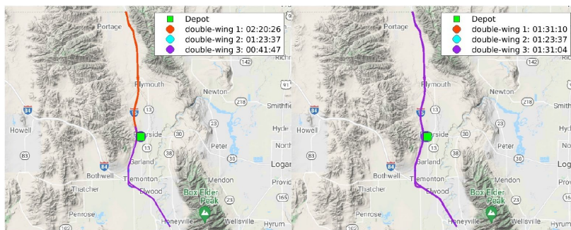
Figure 3.35 (Riverside) UDOT plowing routes (left) and proposed plowing routes (right) along I-15 in group 1 (animation: https://youtu.be/PILQztuc3K8 )
