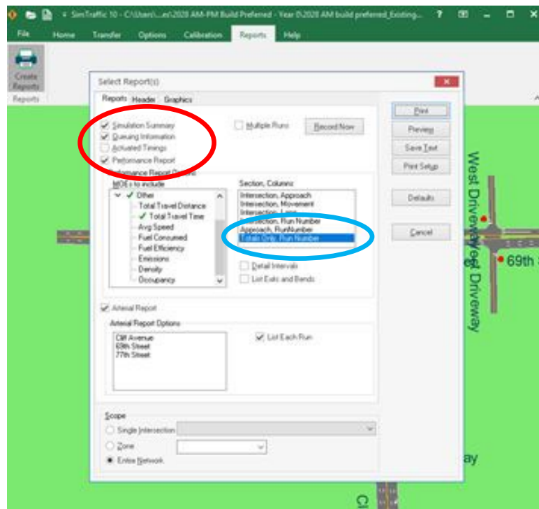
Figure C.4 Obtaining Required Outputs from SimTraffic
