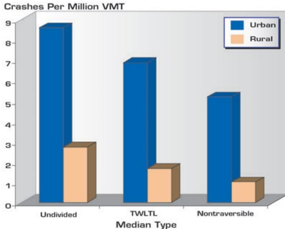
Figure A.24 Median Type Crash Rate Comparison (5)
