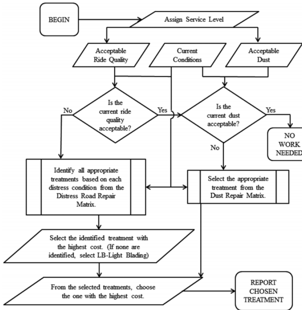
Figure 5.8 WYT2/LTAP Algorithm for Selecting the Best Maintenance Practice (Huntington & Ksaibati, 2011)
