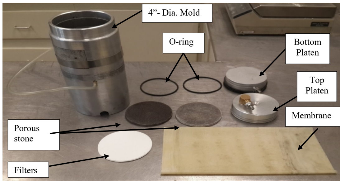
Figure 3.2 Four-inch diameter mold and other apparatus (Mebratom 2017)
