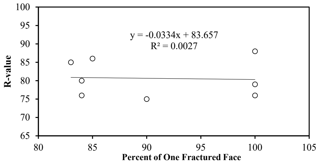
Figure 4.13 R-value versus percent of one fractured face of samples at optimum moisture content
