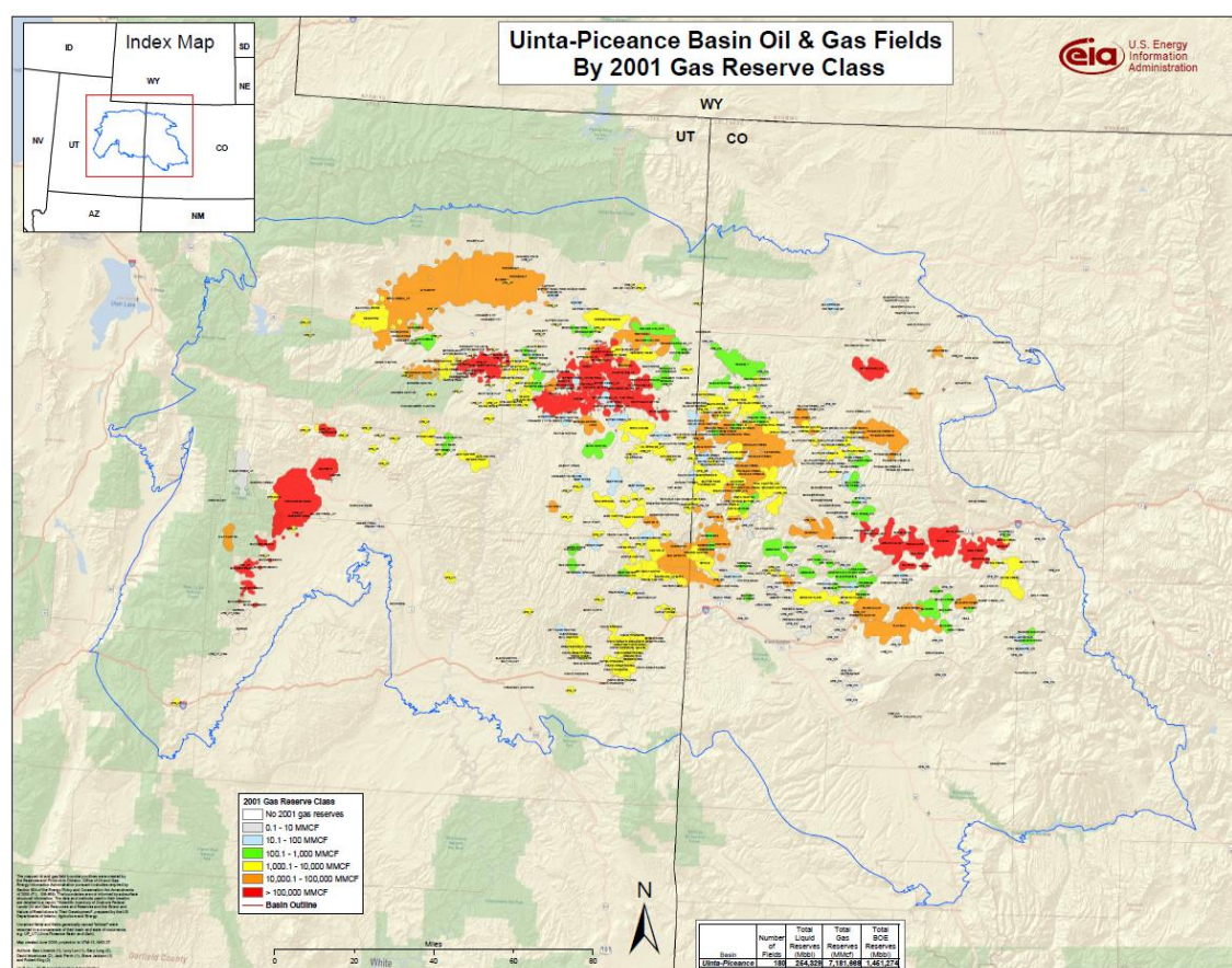
Figure 4.6 Map of the Uinta-Piceance Basin (Source: U.S. EIA)
