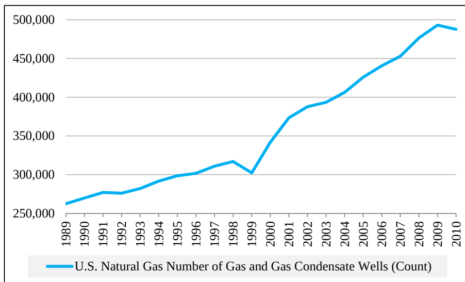
Figure 3.3 U.S. Natural Gas Number of Gas and Gas Condensate Wells (Source: U.S. EIA)
