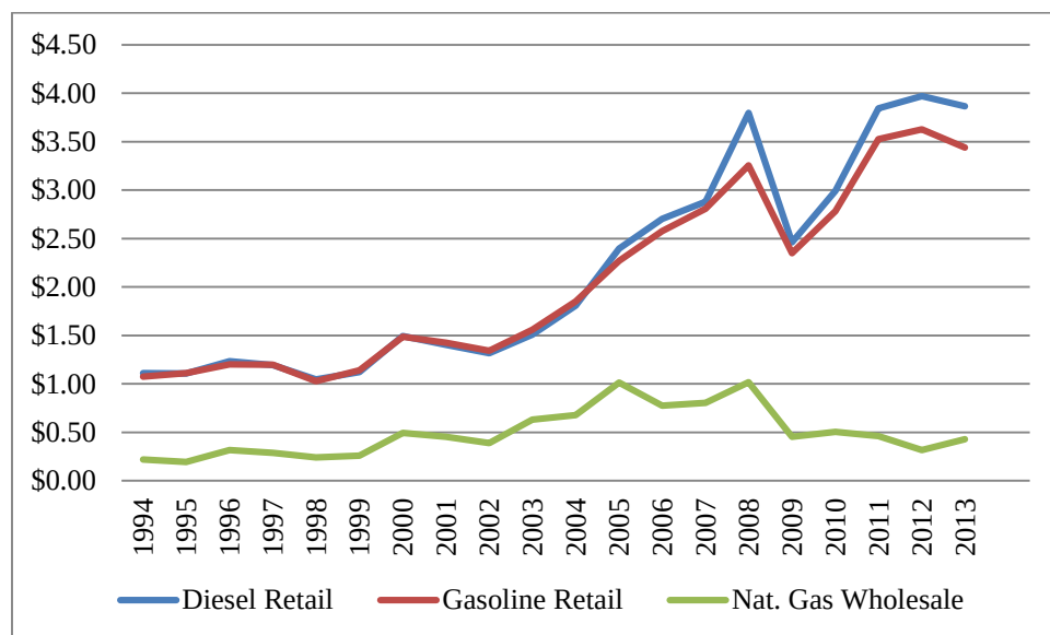
Figure 4.1 Cost of Gasoline, Diesel, and CNG Over Time (Source: U.S. EIA)
