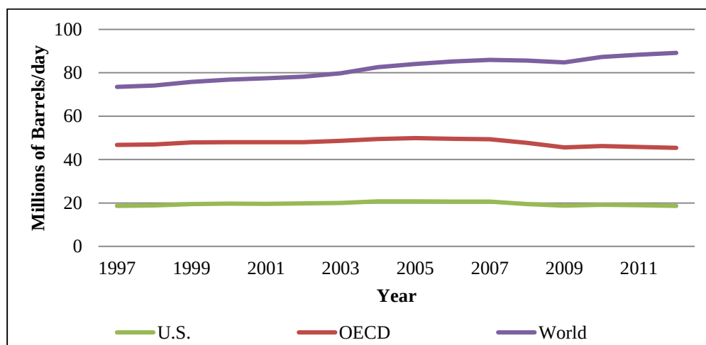
Figure 2.1 World, OECD, and U.S. Oil Demand (U.S. EIA, 2012)
