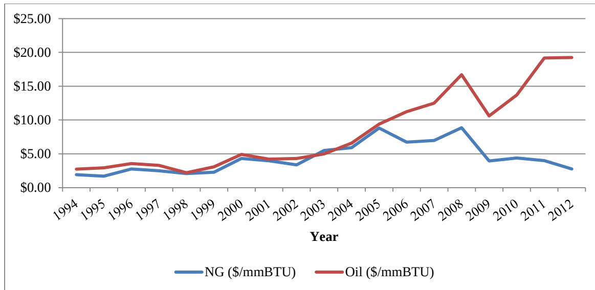
Figure 3.5 Energy Prices (Source: U.S. EIA)
