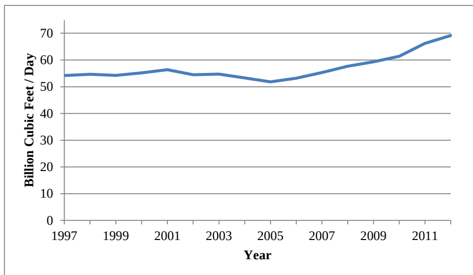
Figure 3.2 U.S. Natural Gas Production (Source: U.S. EIA)
