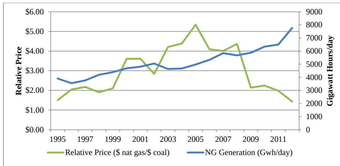
Figure 3.6 Relative Price in Dollars of Natural Gas to Coal and NG Generation
