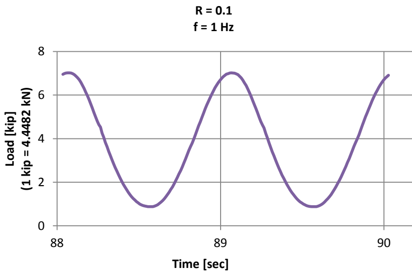
Figure 3.2 Typical pulsating load (Specimen F10)
