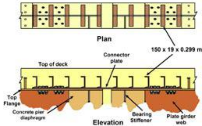
Figure 1.6 Detail of connection plate on top flanges on NM 187 bridge [5].
