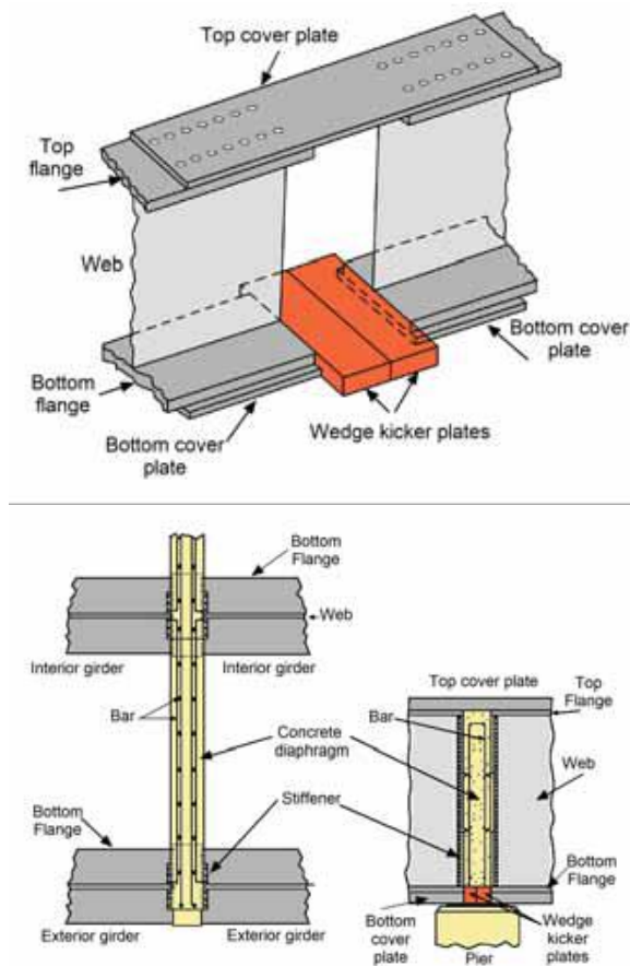
Figure 1.4 Tennessee design detail for continuity at pier [17].
