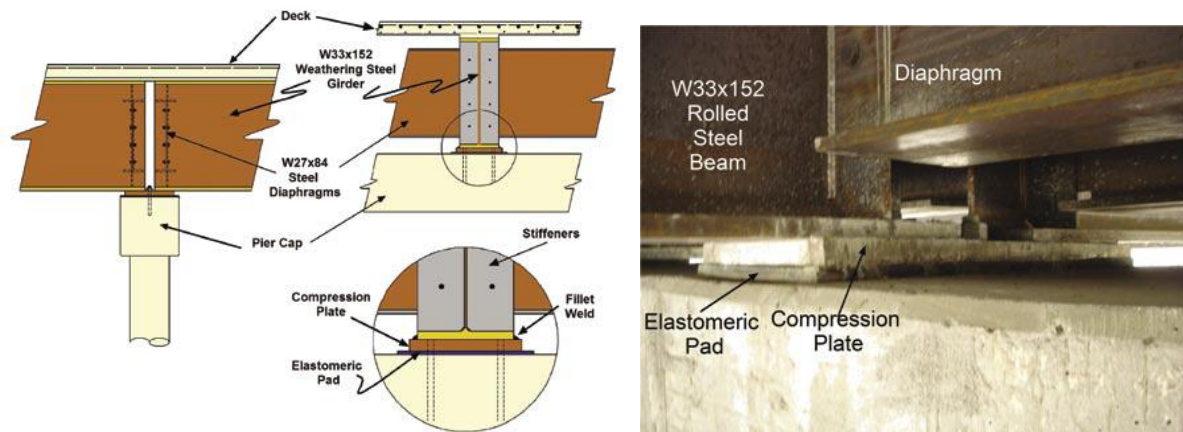
Figure 1.7 Colorado beam continuity connection above pier cap [16].
