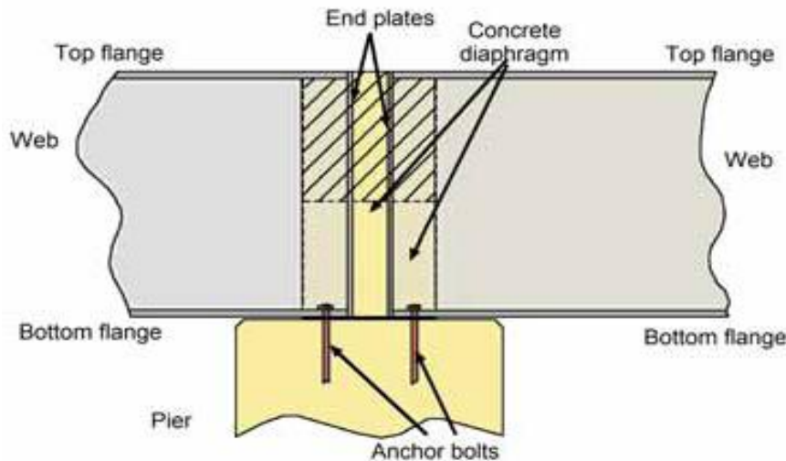
Figure 1.3 Initial Tennessee beam connection [17].
