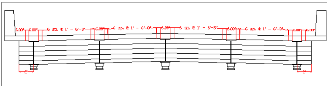
Concrete Diaphragm at Pier
