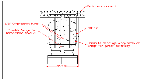
Stage 2 Concrete Diaphragm
