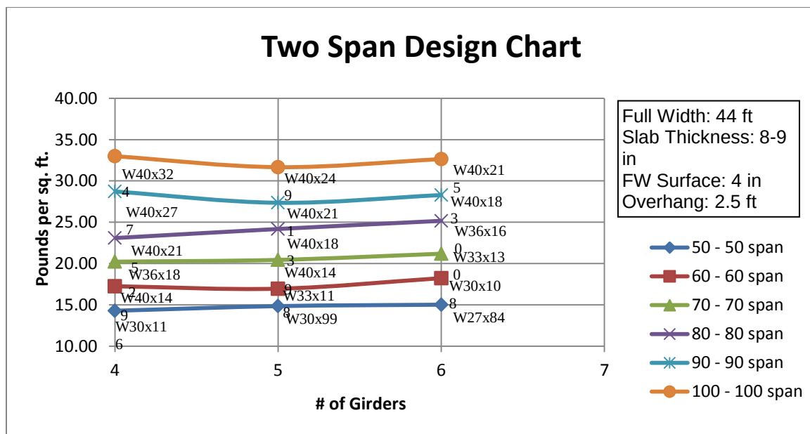
Figure 4.1 Example of a Two Span Design Chart.
