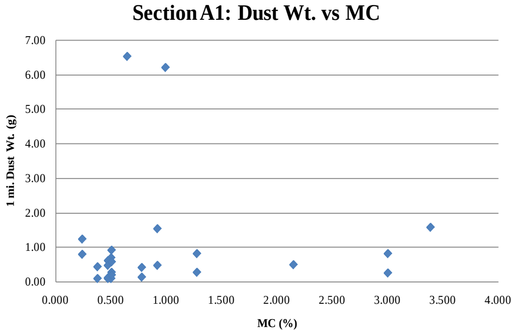
Figure 5.4 Example from Laramie County Dust vs. Moisture Content
