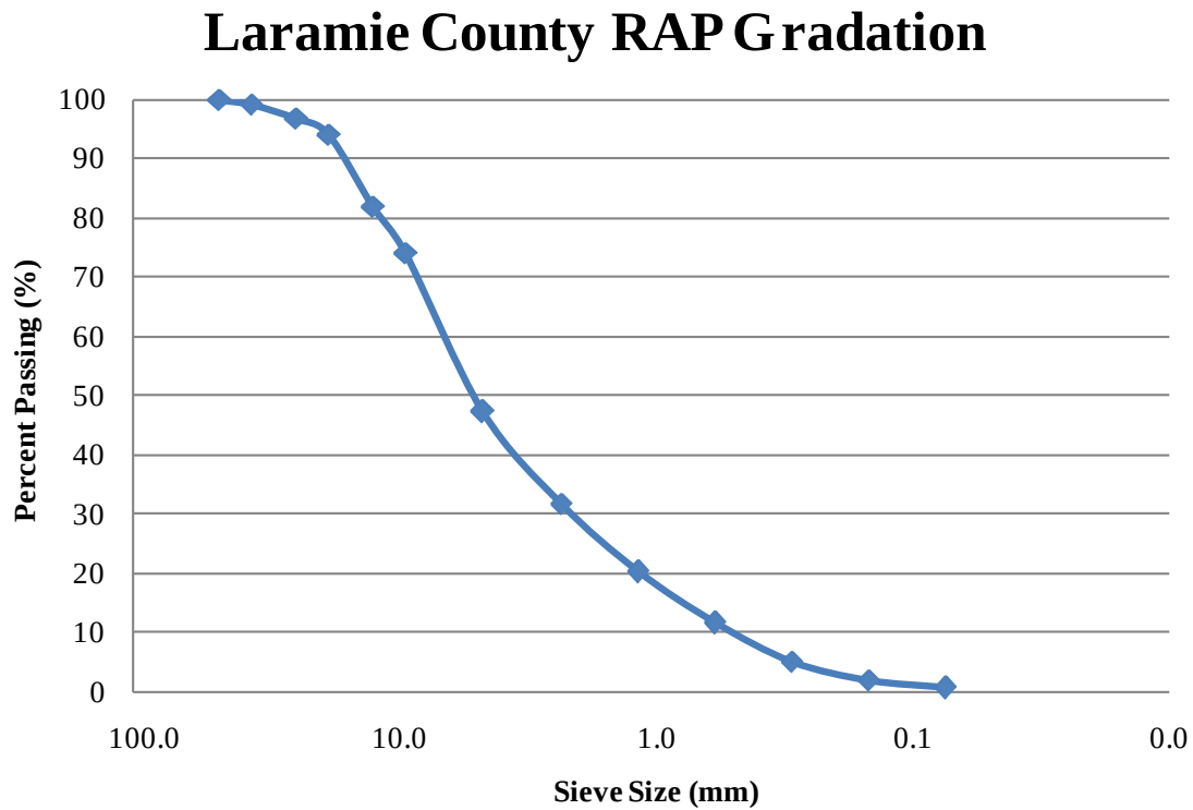
Figure 4.1 Gradation of RAP Material Used in Laramie County.
