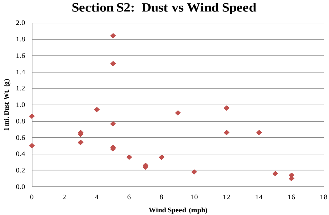
Figure 5.5 Example from Johnson County Dust vs. Wind Speed
