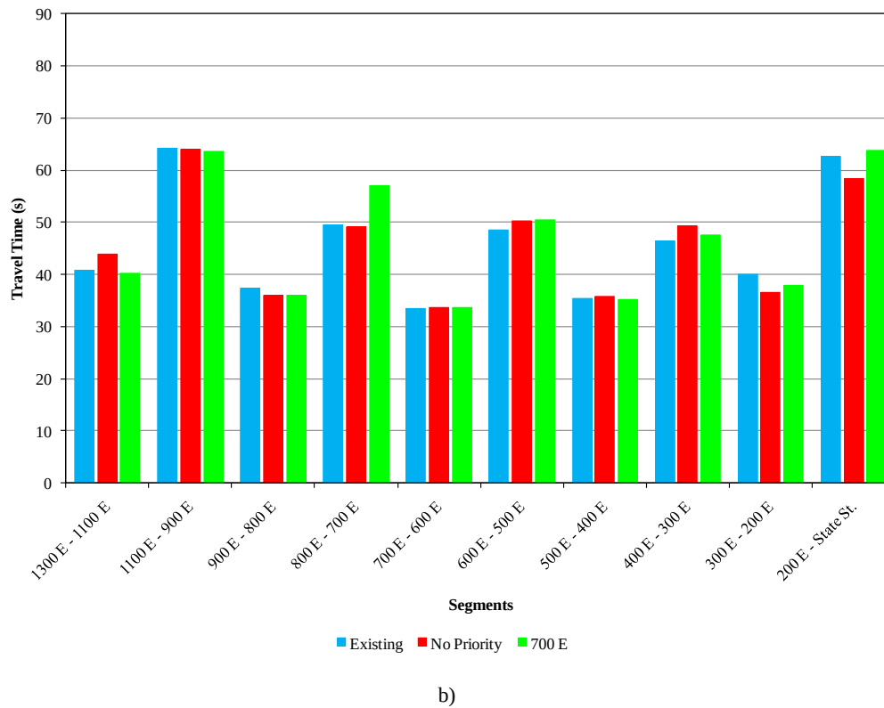
Figure 5.1 Vehicular Travel Times Comparison – Model Scenarios: a) Eastbound; b) Westbound
