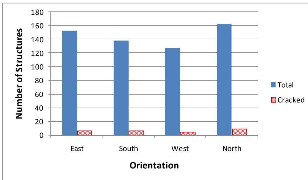
Figure 4.5 WPC-2 Orientations and Cracking Status
