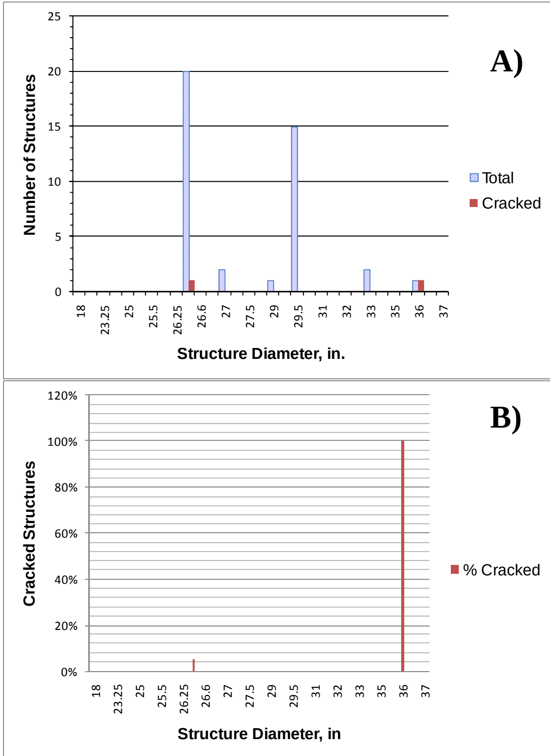
Figure 4.42 WPC-3 Base Diameter A) Cracking Status and B) Percent Cracked
