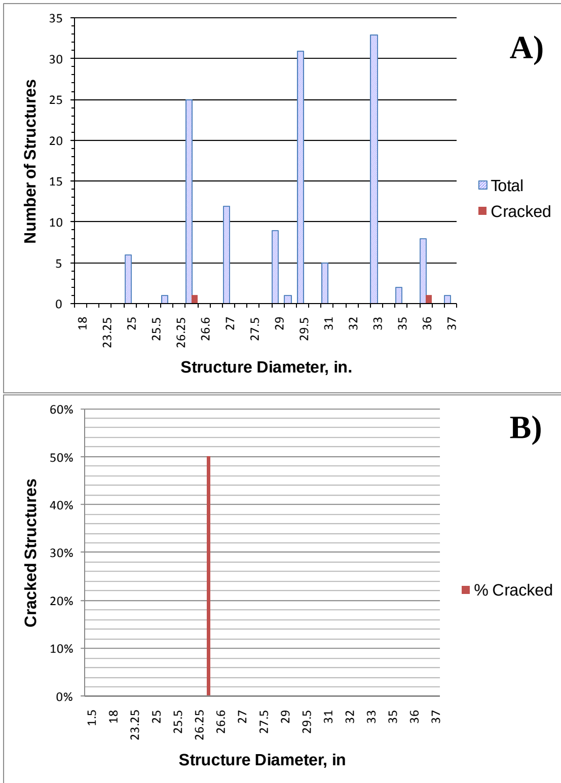
Figure 4.43 WPC-4 Base Diameter A) Cracking Status and B) Percent Cracked
