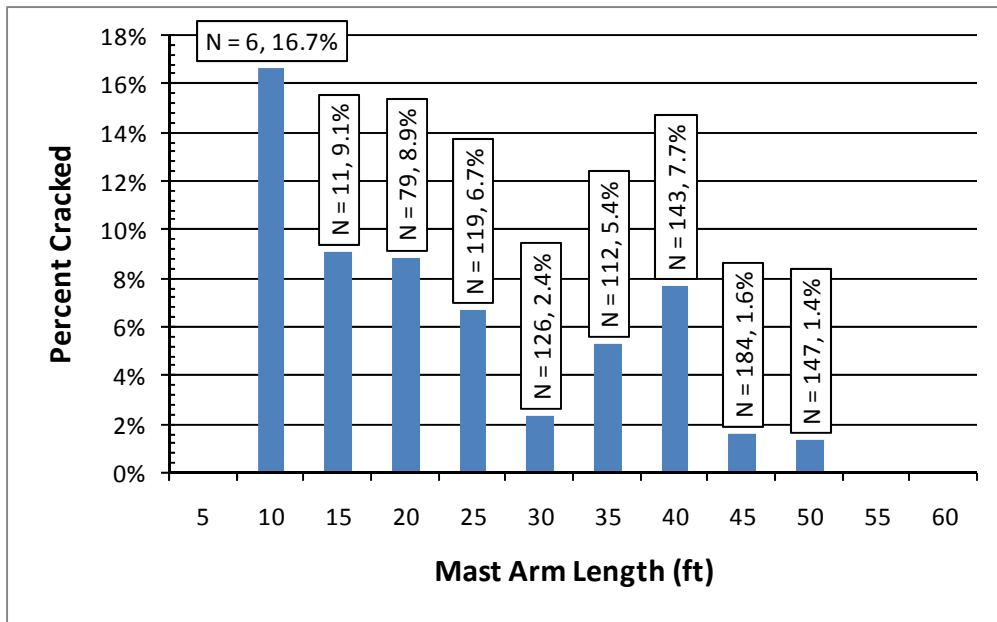
Figure 4.16 Percent of Structures cracked in WPC-1 by Mast-Arm Lengths
