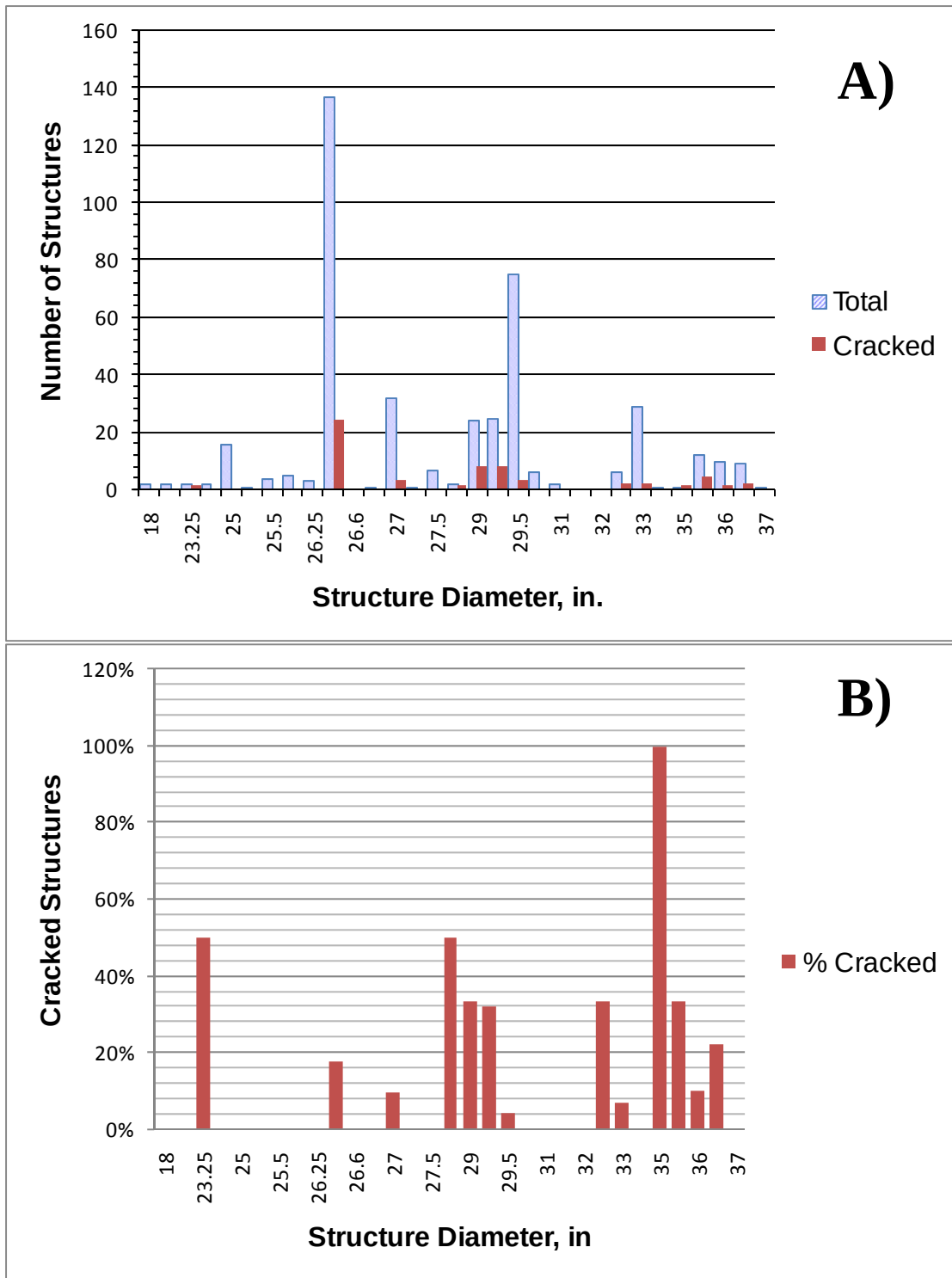
Figure 4.41 WPC-2 Base Diameter A) Cracking Status and B) Percent Cracked
