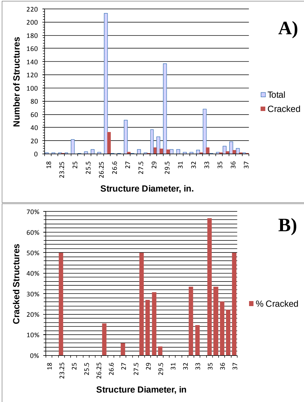
Figure 4.40 All WPCs Base Diameter A) Cracking Status and B) Percent Cracked
