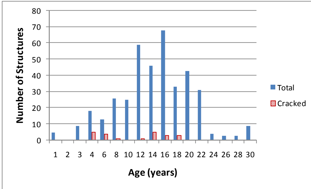
Figure 4.23 Age and Cracking Status for WPC-2
