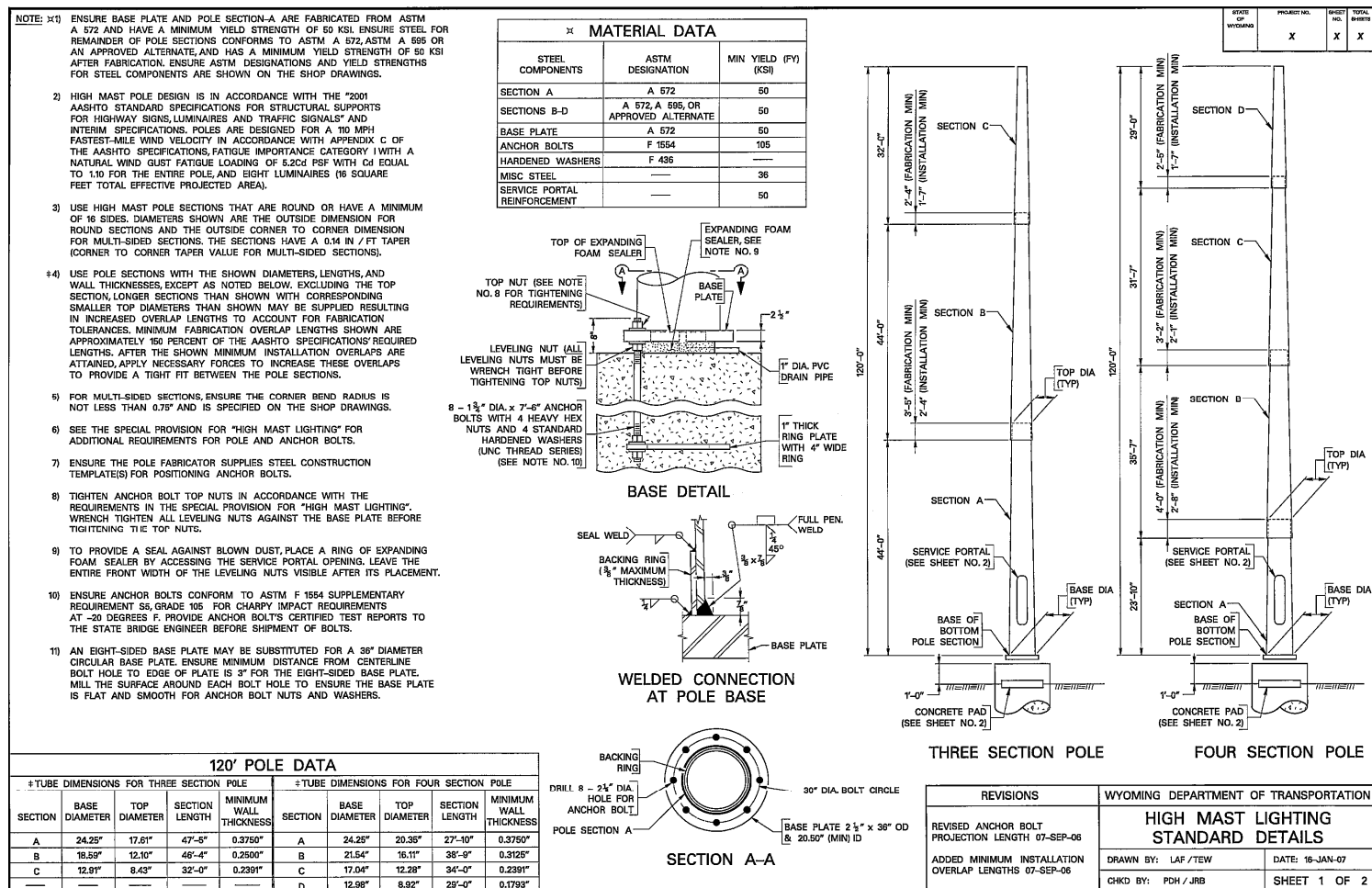
Figure D.3 Typical WYDOT Pole Plan Set
