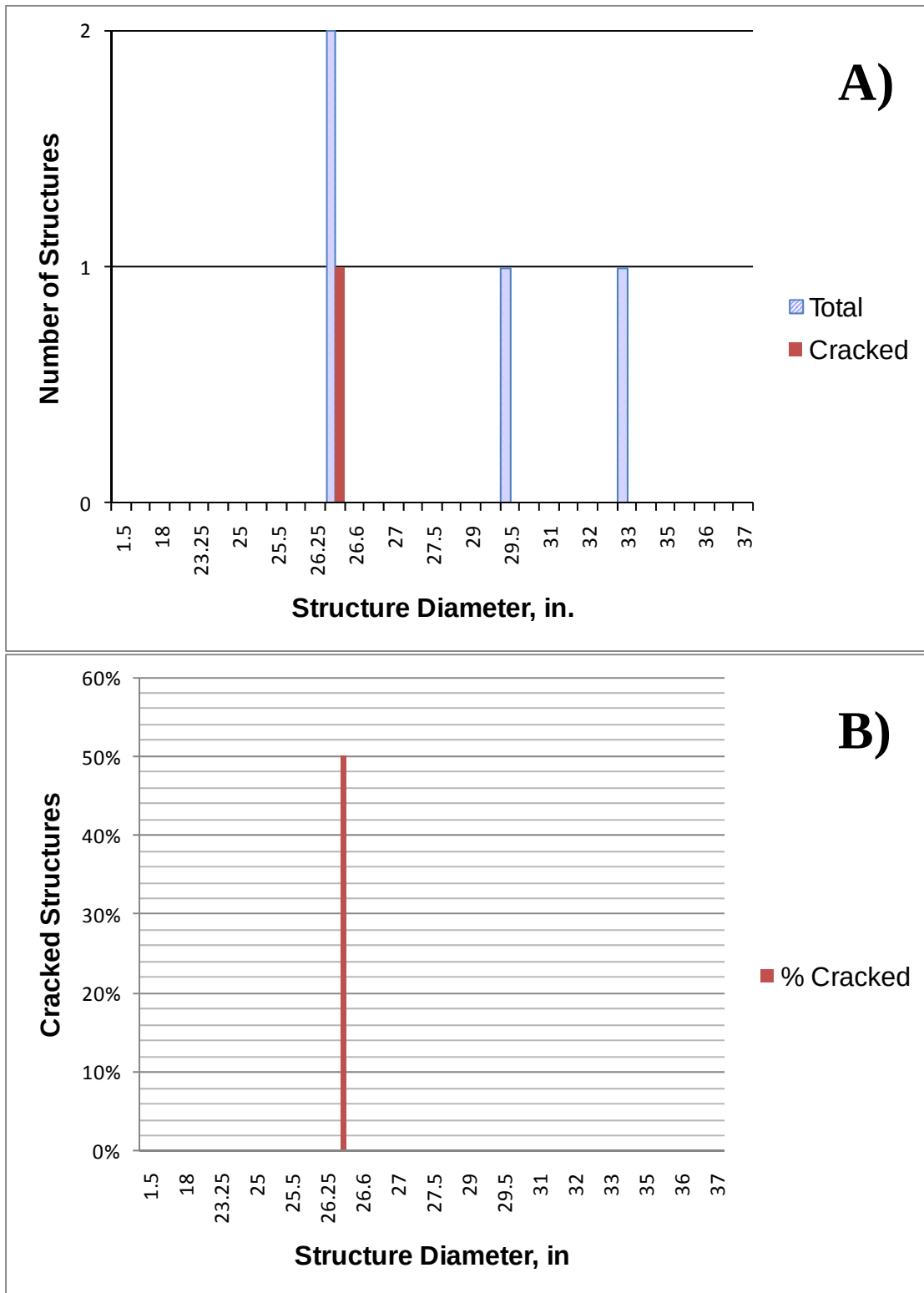
Figure 4.44 WPC-5 Base Diameter A) Cracking Status and B) Percent Cracked
