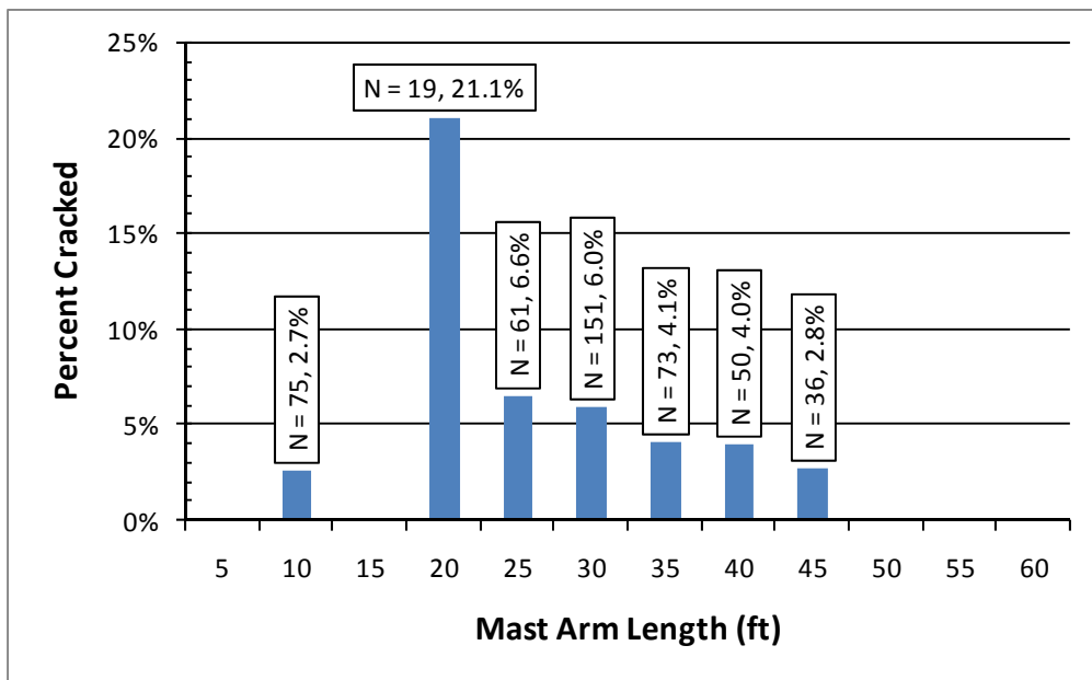
Figure 4.17 Percent of Structures Cracked in WPC-2 by Mast-Arm Lengths
