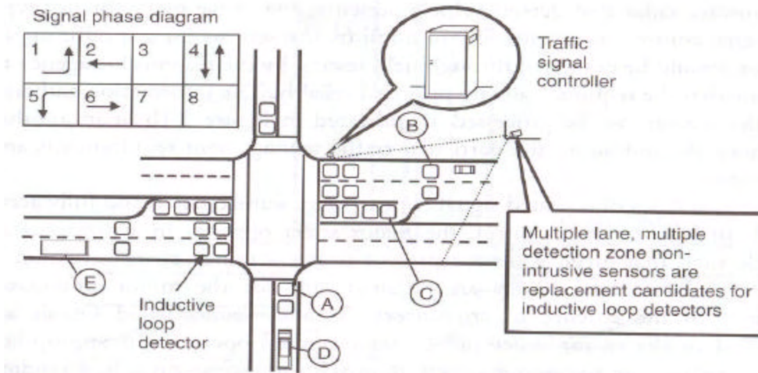
Figure 3.1: Actuated Isolated Intersection Signal Control
