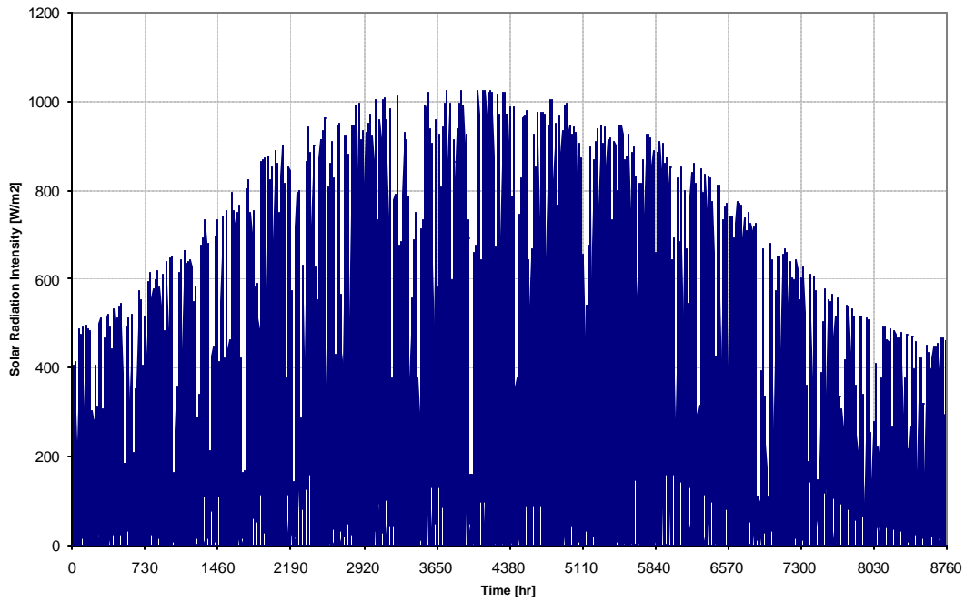
Figure 13 Denver, Colo., TMY Global Solar Radiation
