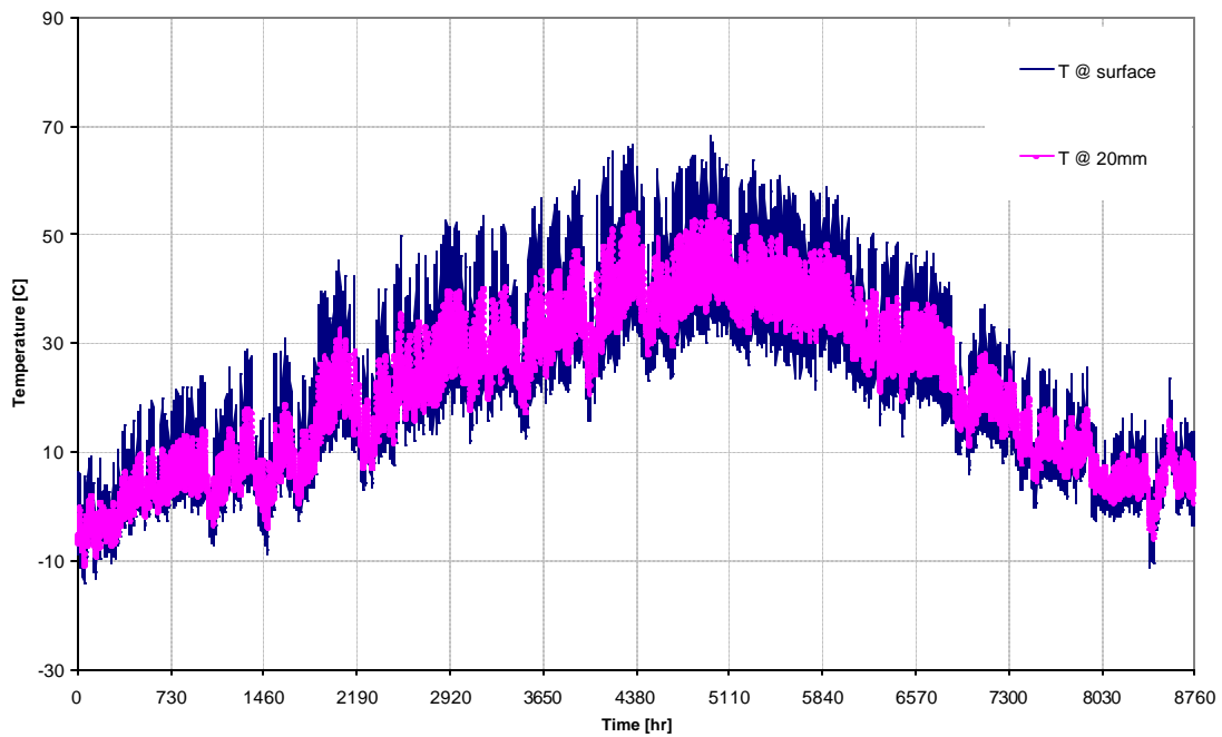
Figure 14 Denver, Colo., Asphalt Temperature Predictions
