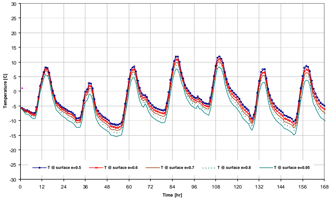
Figure 21. Sensitivity of Temperature Predictions to Emissivity of Asphalt Material using Denver, Colo., minimum Temperatures Predictions
