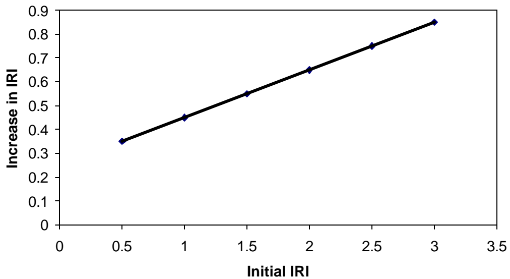
Figure 5.7 DIRI Variations (Increase in IRI) versus Initial IRI for Asphalt Sections
