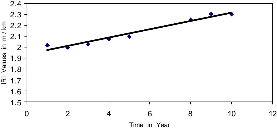
Figure 5.9 Variations in IRI Values over Time for Concrete Sections 29-5000 from Missouri
