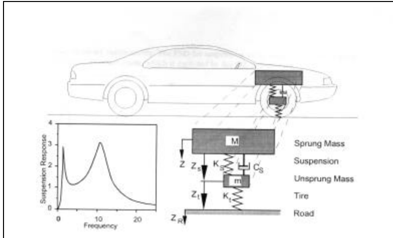
Figure 2.1 The Quarter Car Model
