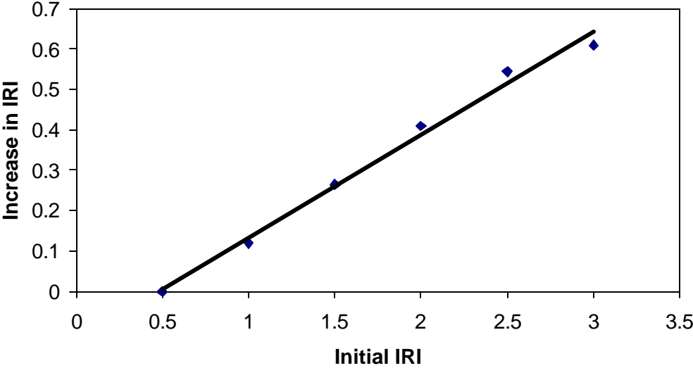
Figure 5.14 DIRI Variations (Increase in IRI) versus Initial IRI for Concrete Sections
