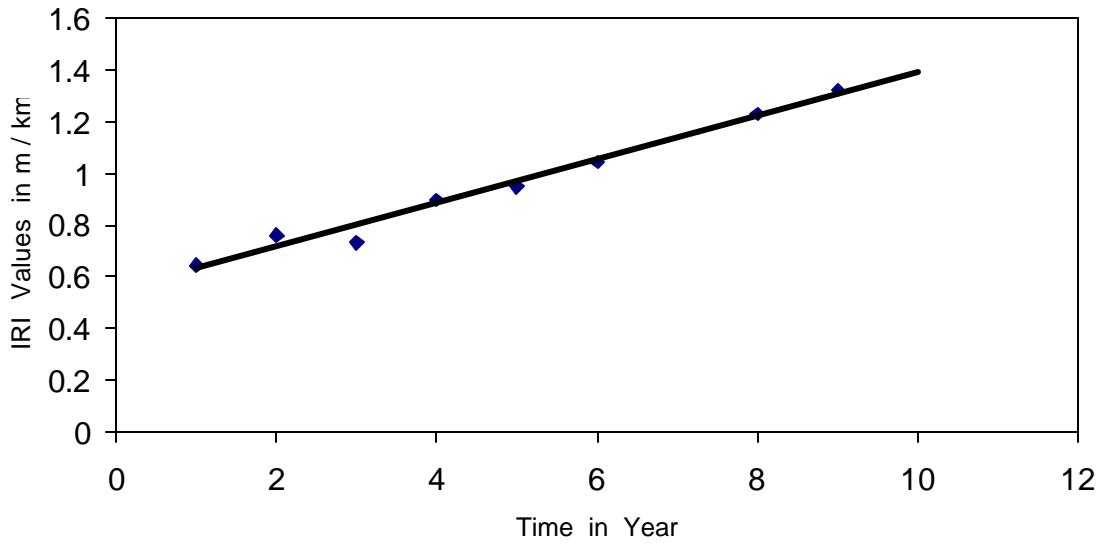
Figure 5.1 Variations in IRI Values over Time for Asphalt Section 46-9187 from South Dakota
