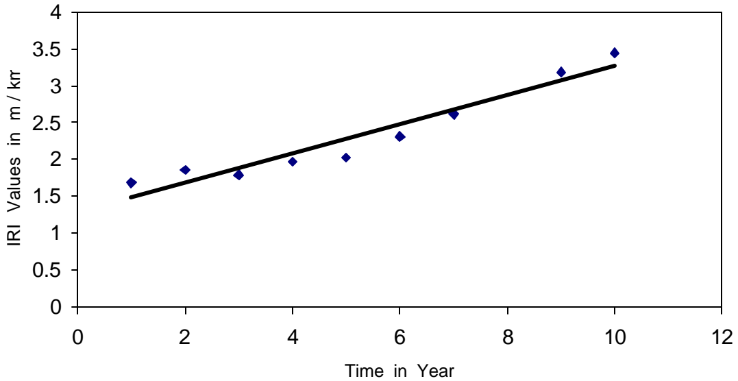
Figure 5.2 Variations in IRI Values over Time for Asphalt Section 42-1597 from Pennsylvania
