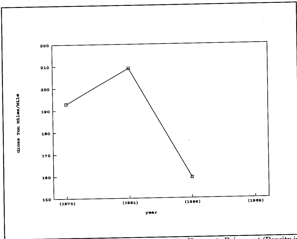
Figure 120: Burlington Northern Line Segment 071, Havana to Fairmount (Density in Thousands of Gross Ton Miles per mile)
