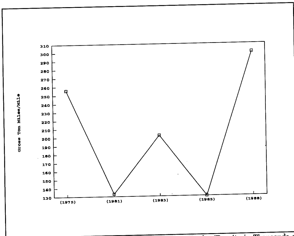
Figure 136: Soo Line Segment 125, Flaxton to East Westby (Density in Thousands of Gross Ton Miles per mile)
