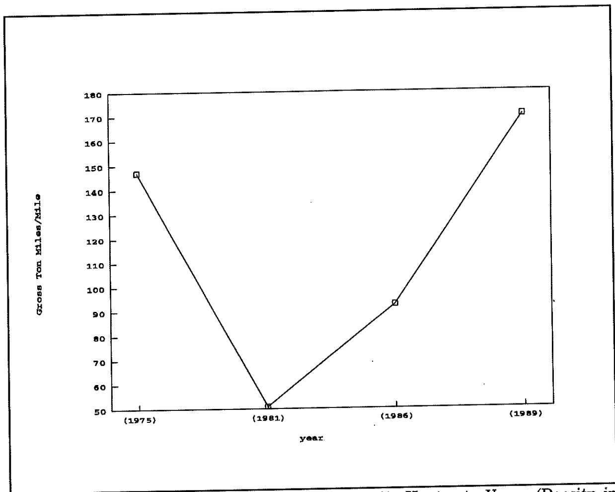
Figure 108: Burlington Northern Line Segment 043, Hunter to Vance (Density in Thousands of Gross Ton Miles per mile)
