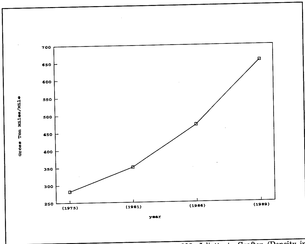
Figure 96: Burlington Northern Line Segment 033, Joliet to Grafton (Density in Thousands of Gross Ton Miles per mile)
