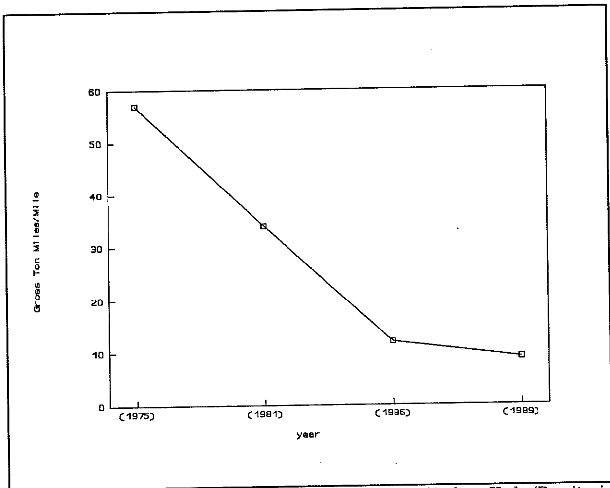
Figure 75: Burlington Northern Line Segment 015, Wolford to York (Density in Thousands of Gross Ton Miles per mile)
