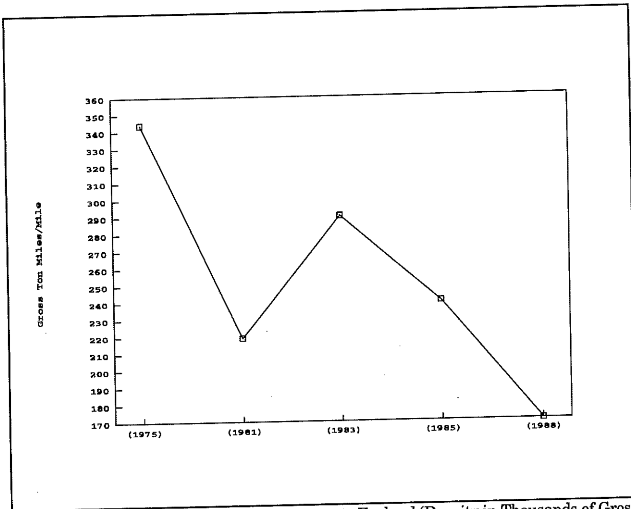
Figure 151: Soo Line Segment 135, Kenmare to Egeland (Density in Thousands of Gross Ton Miles per mile)
