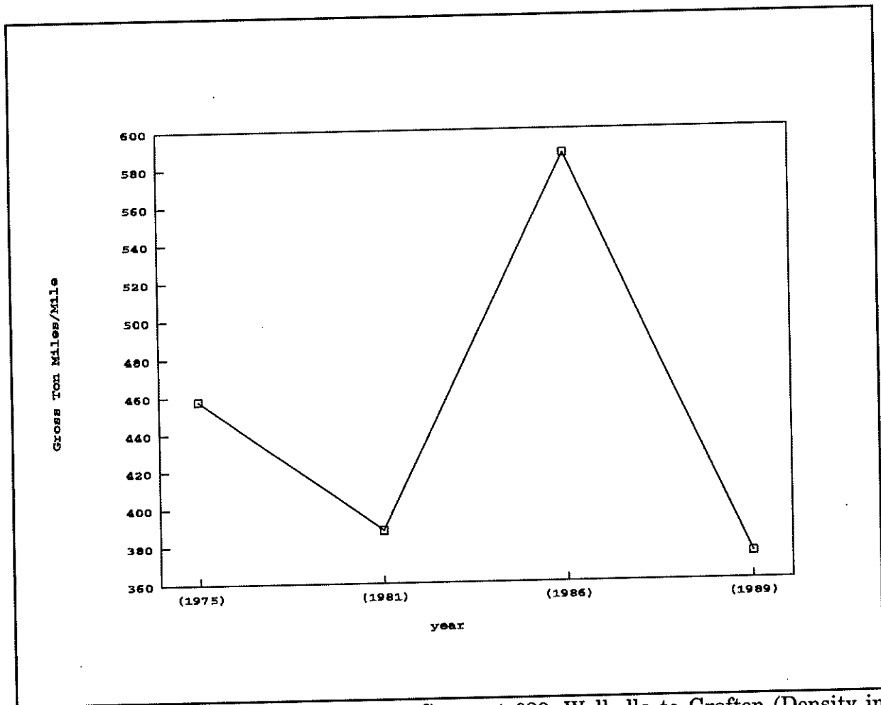
Figure 90: Burlington Northern Line Segment 029, Walhalla to Grafton (Density in Thousands of Gross Ton Miles per mile)
