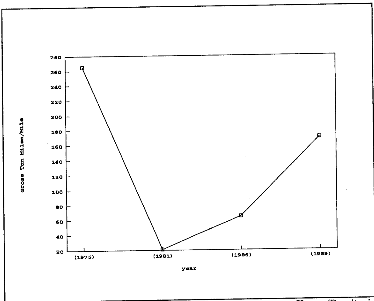
Figure 133: Burlington Northern Line Segment 115, Amenia to Vance (Density in Thousands of Gross Ton Miles per mile)
