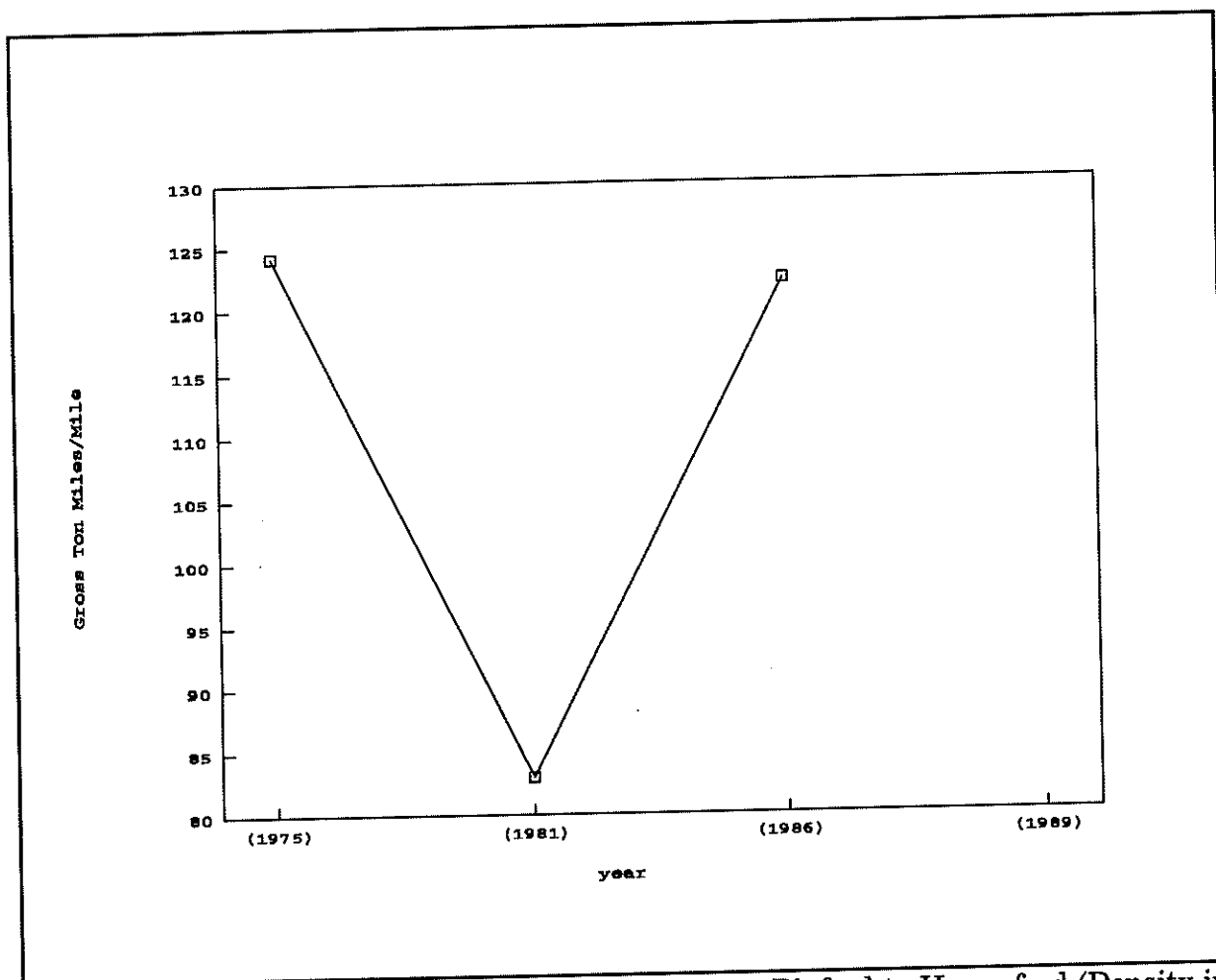
Figure 105: Burlington Northern Line Segment 039, Binford to Hannaford (Density in Thousands of Gross Ton Miles per mile)
