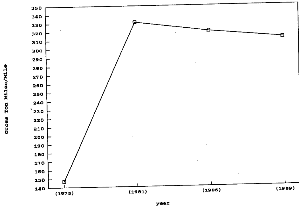
Figure 123: Burlington Northern Line Segment 073, Mayville to Larimore (Density in Thousands of Gross Ton Miles per mile)
