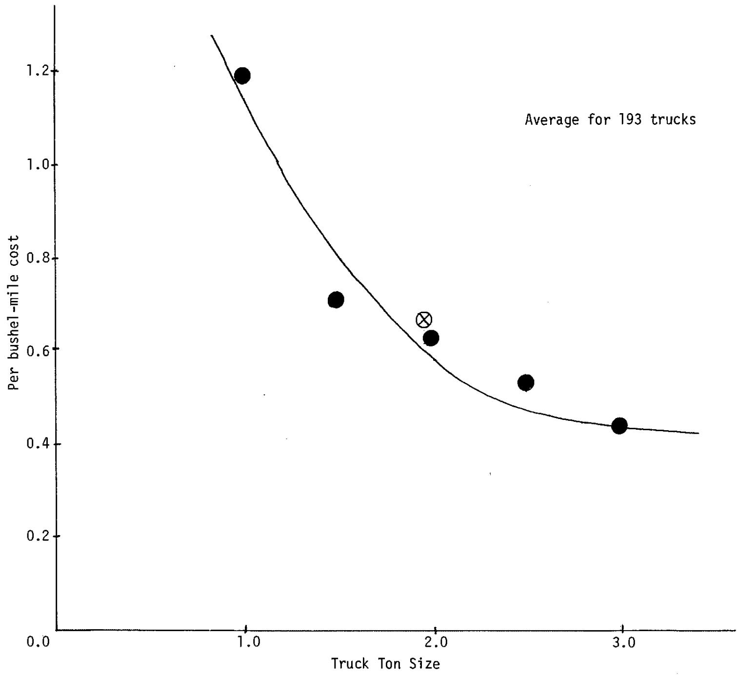
Figure 5. Relationship Between Truck Tonnage and Bushel-Mile Costs.
