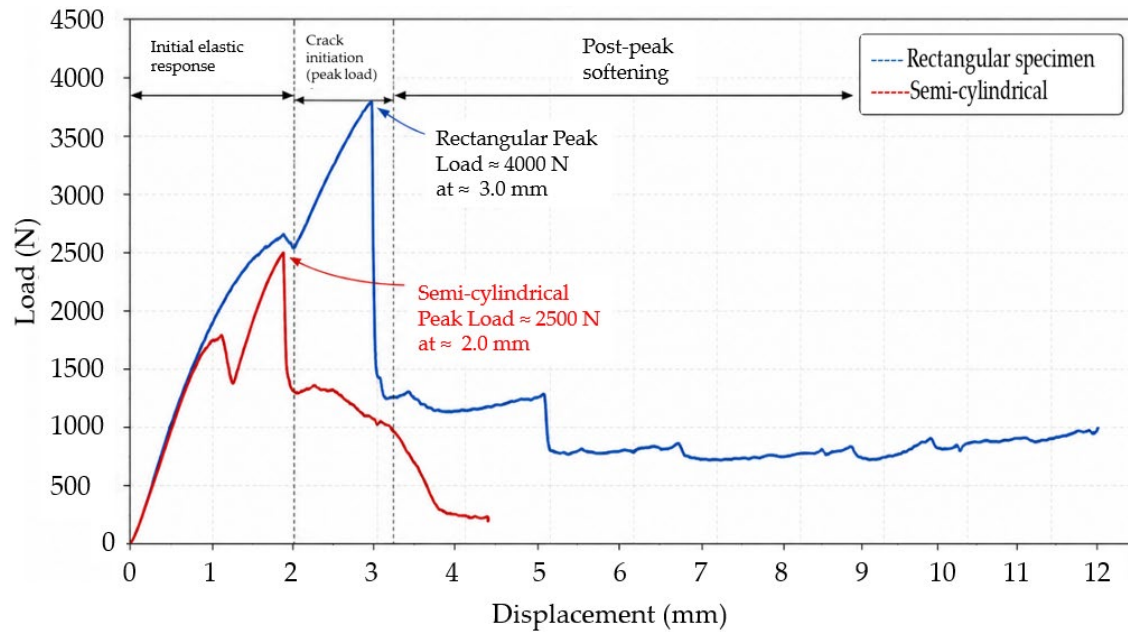
Figure 13. Experimental load–displacement responses of the rectangular and semi-cylindrical specimens subjected to three-point bending
