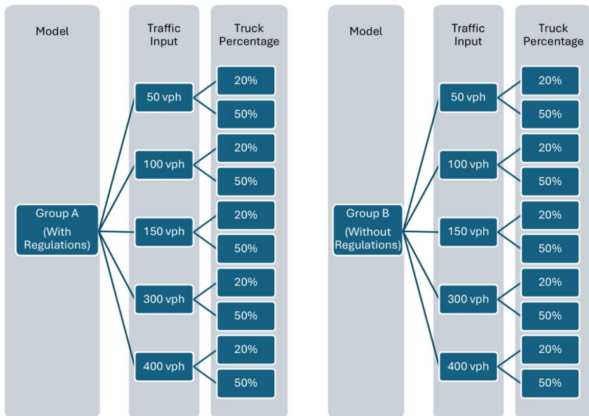
Figure 19: Simulation scenarios
