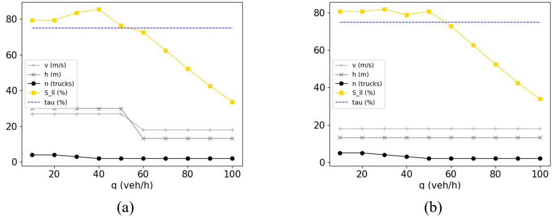
Figure 10: Change in platooning rules and the estimated lower limit of safety ratio, S_{II} , with the opposite direction traffic flow rate, q . Weights: (a) w_v = w_h = w_n = 1 . (b) w_v = w_h = 1, w_n = 0.6 .
