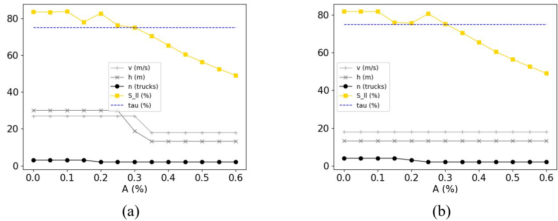
Figure 12: Change in platooning rules and the estimated lower limit of safety ratio, S_{II} , with the vertical curve grade difference, A . Weights: (a) w_v = w_h = w_n = 1 . (b) w_v = w_h = 1, w_n = 0.6 .
