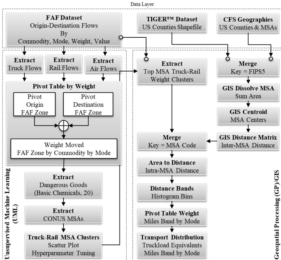
Figure 58: The HDM workflow to analyze hazardous material flows
