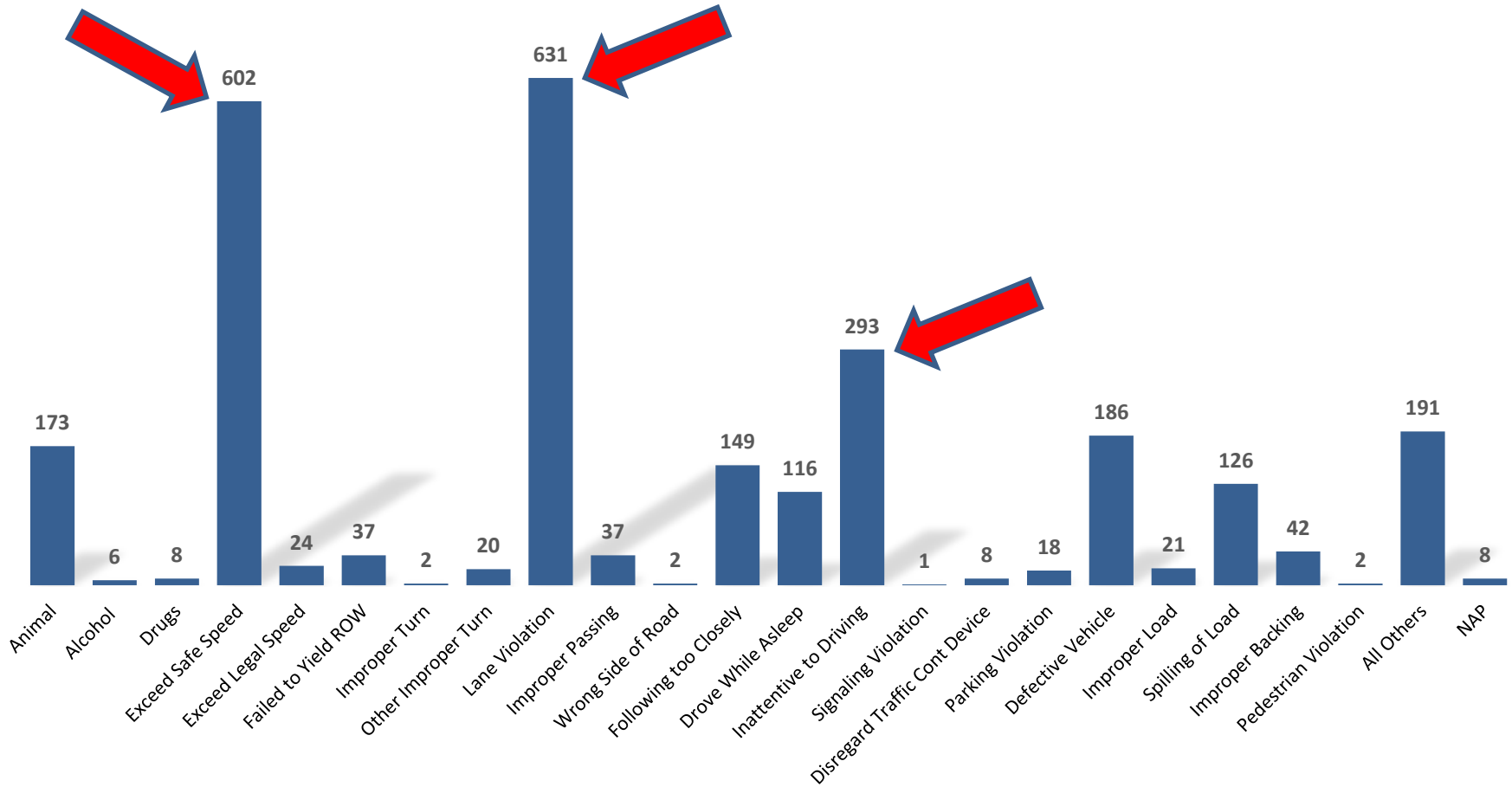
I-70 Causal Factors - CMV-Caused
