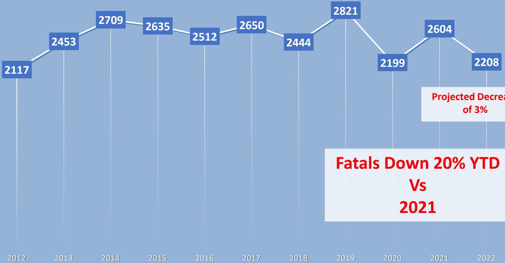
CMV-INVOLVED CRASHES
