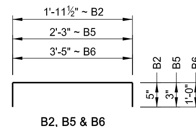
BENT BAR DETAILS
