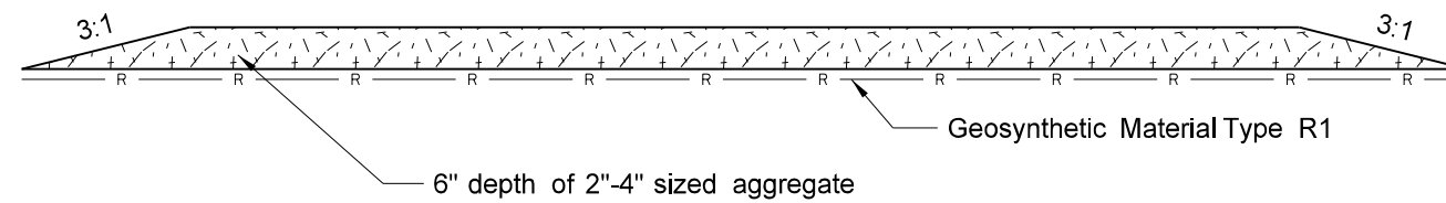
A - A Cross Section
