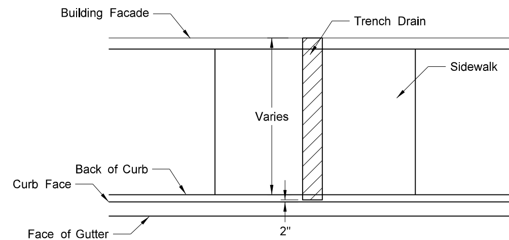
Trench Drain Layout
