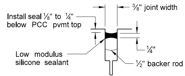
Transverse Joint Seal
