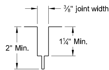
Transverse Joint Sawing
