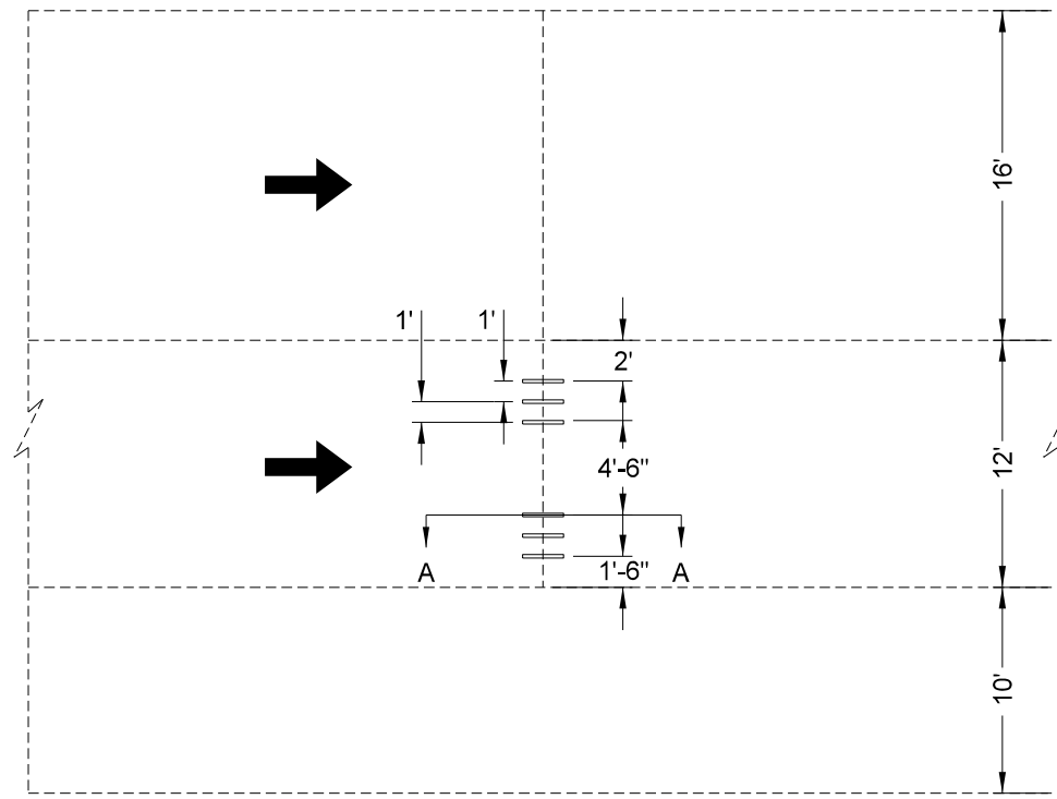
Dowel Bar Retrofit Spacing
