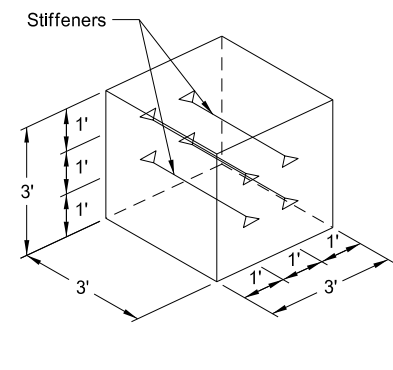
Interior Gabion Cells
