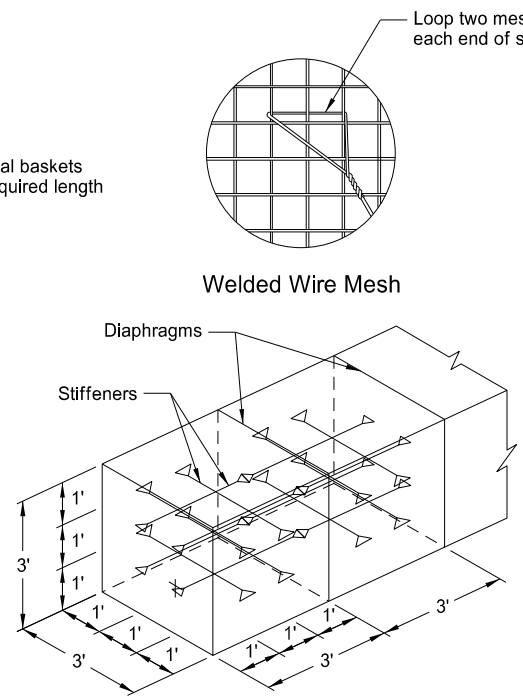
End Gabion Cells
