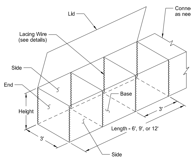
Typical Assembled Gabion Basket
