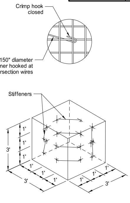
All Gabion Cells Optional Gabion Stiffeners (welded wire baskets)
