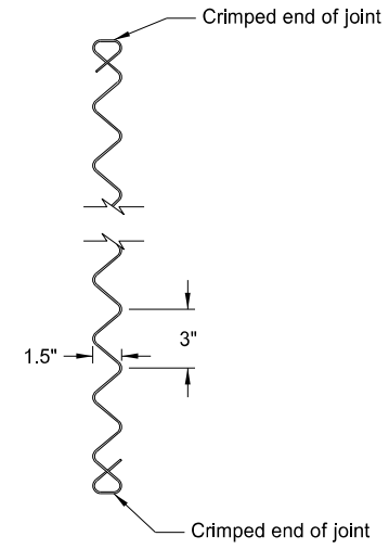
0.150" Diameter Spiral Fastener
