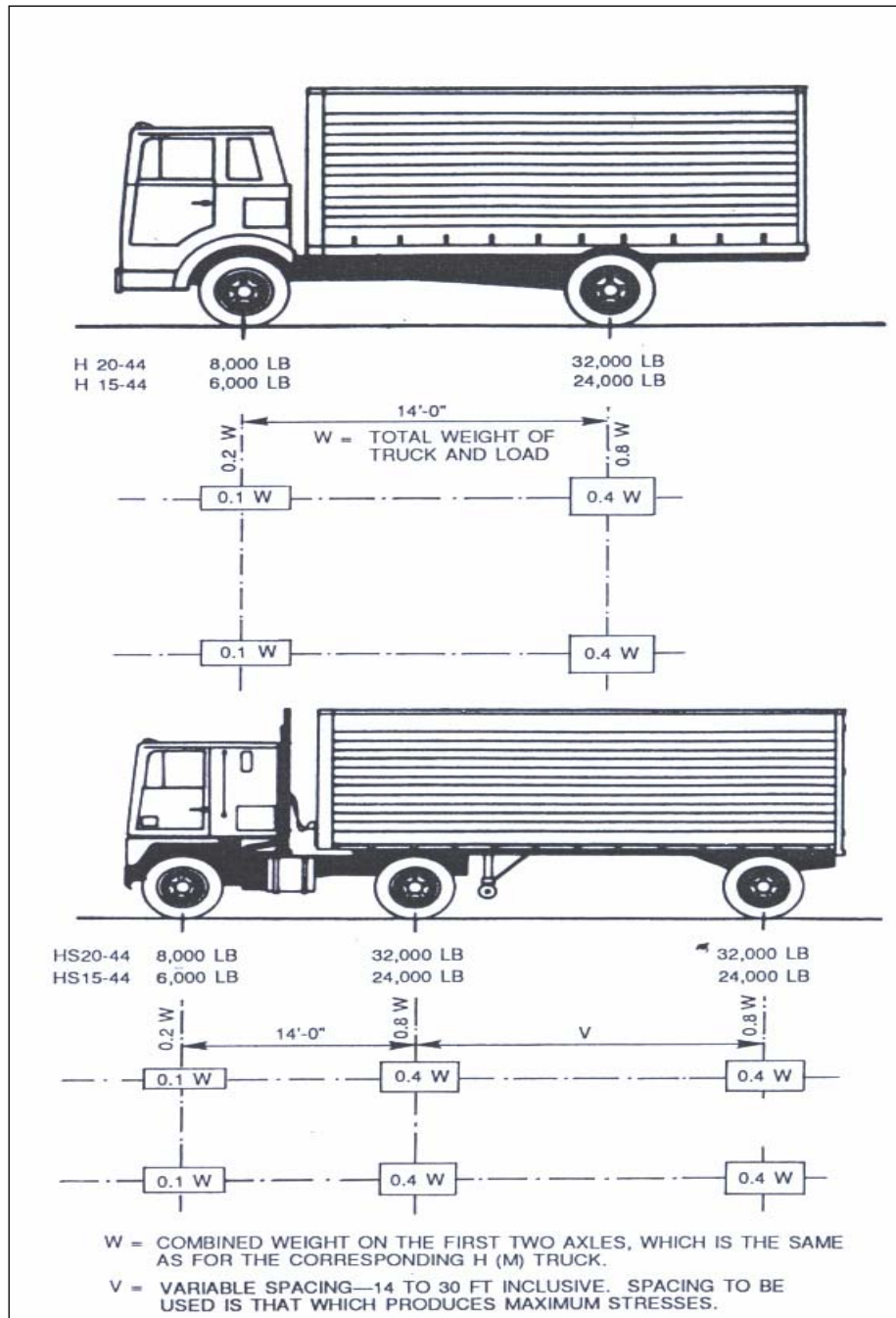
Figure 17. AASHTO Design Vehicles. (Source: Truck Weight Limits, Special Report 225)
