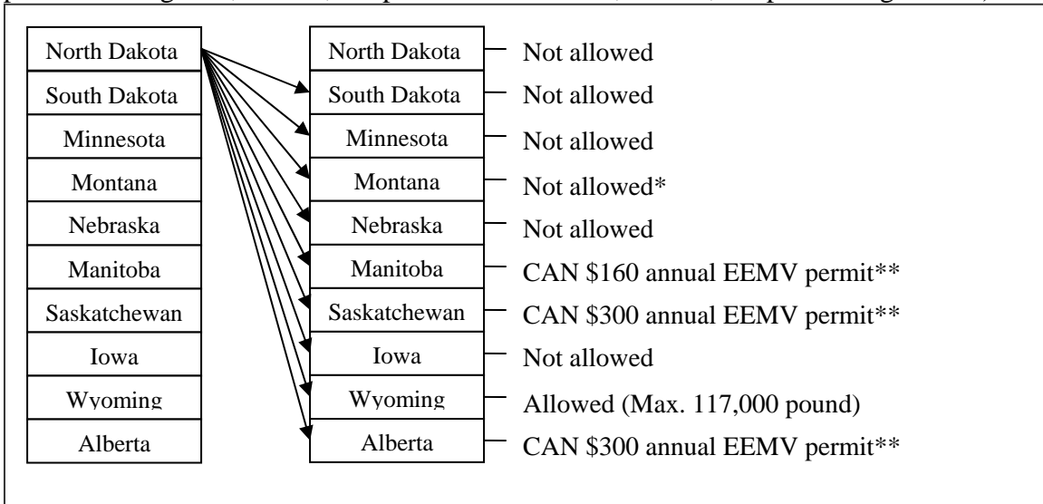
Figure 43. Scenario for a Rocky Mountain Double (7 axles, 105,500 pounds, 12,000 pound steering axle, two 35,000 pound tandem axles, two 11,750 pound single axles).
