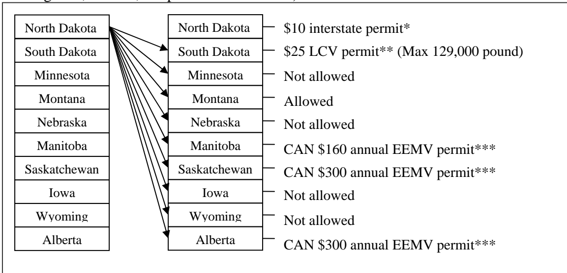
Figure 44. Scenario for Turnpike Double (9 axles, 105,500 pounds, 12,000 pound steering axle, four 23,375 pound tandem axles).
