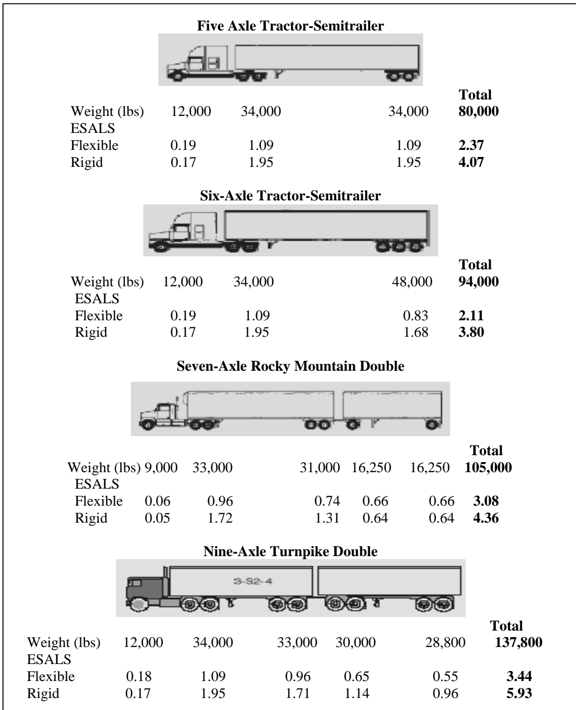
Figure 13. Equivalent Single Axle Loads* (ESAL).
