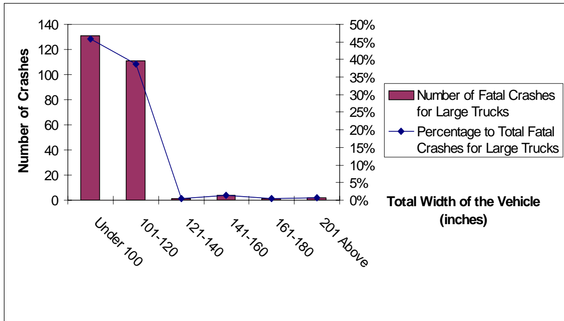
Figure 35. Number of Fatal Crashes for Large Trucks by Total Width of the Vehicle in the Region (No Canadian Provinces) in 2000 (Source: TIFA).
