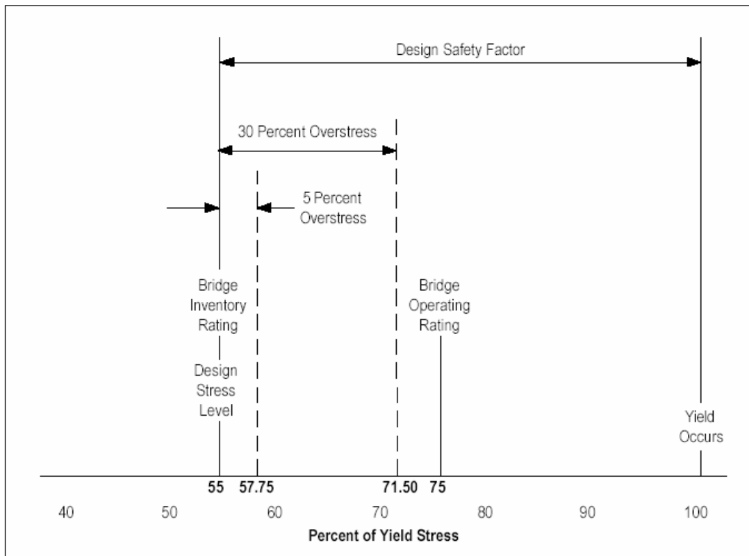
Figure 18. Relationship of Overstress Criteria to Design Stress and Bridge Ratings. (Source: Comprehensive Truck Size and Weight (CTS&W) Study, 2000)
