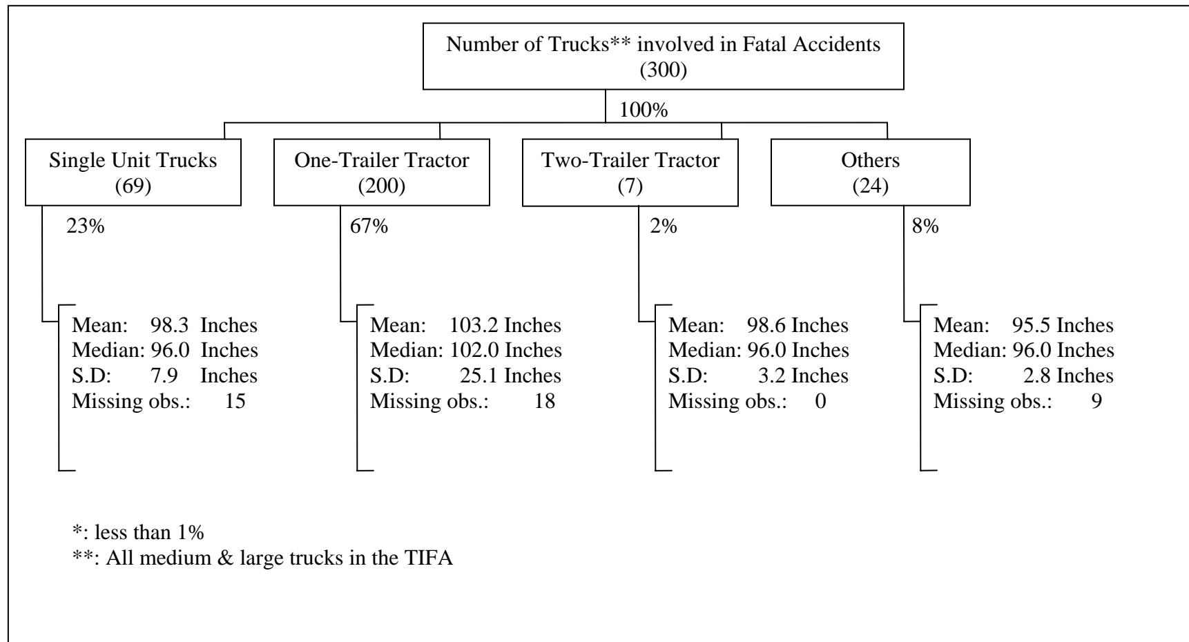
Figure 25. Number of Trucks Involved in Fatal Accidents by Total Width of Vehicle in the Region (No Canadian Provinces) in 2000. (Source: TIFA)
