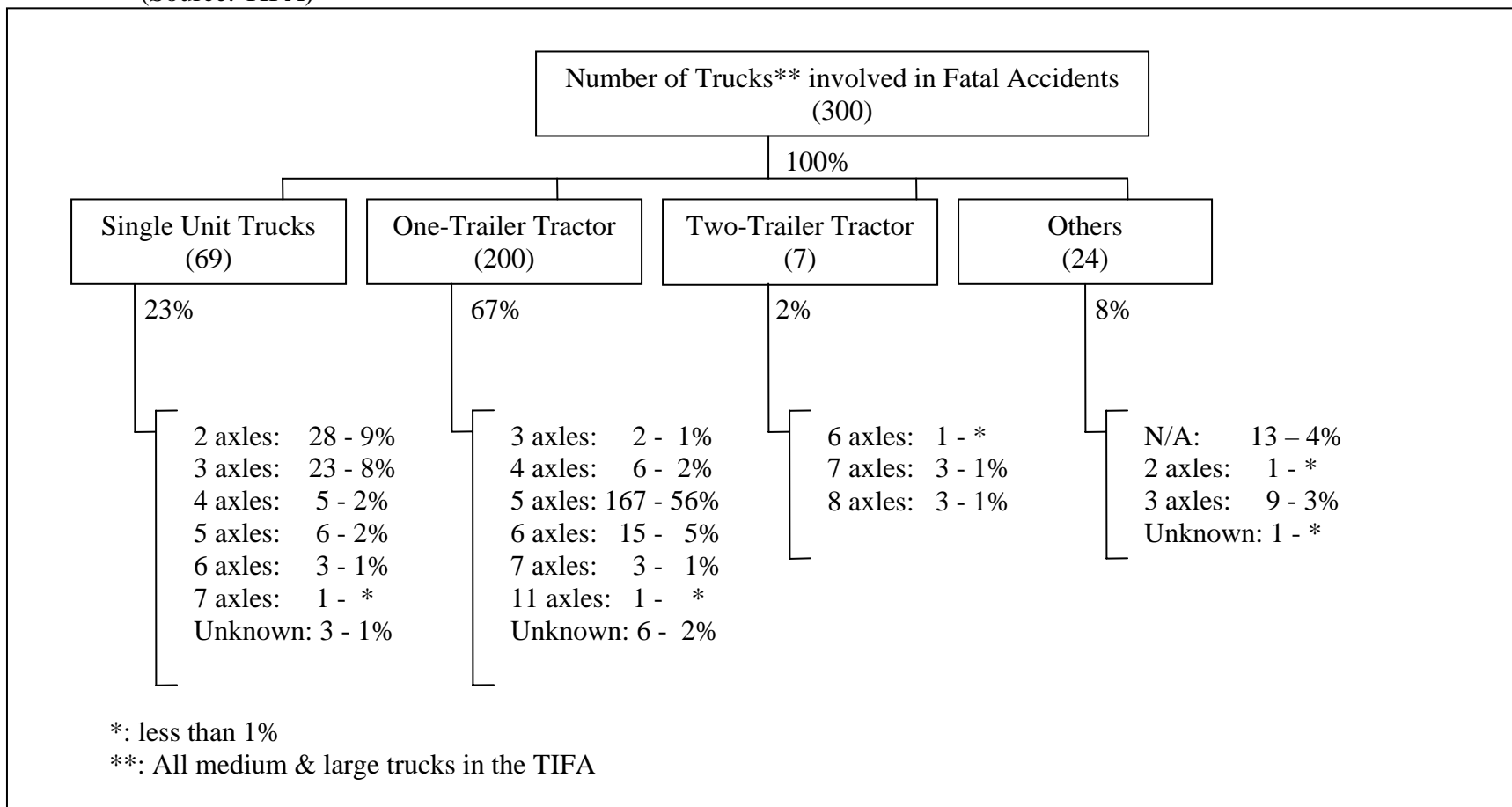
Figure 26. Number of Trucks Involved in Fatal Accidents by Number of Axle in the Region (No Canadian Provinces) in 2000. (Source: TIFA)
