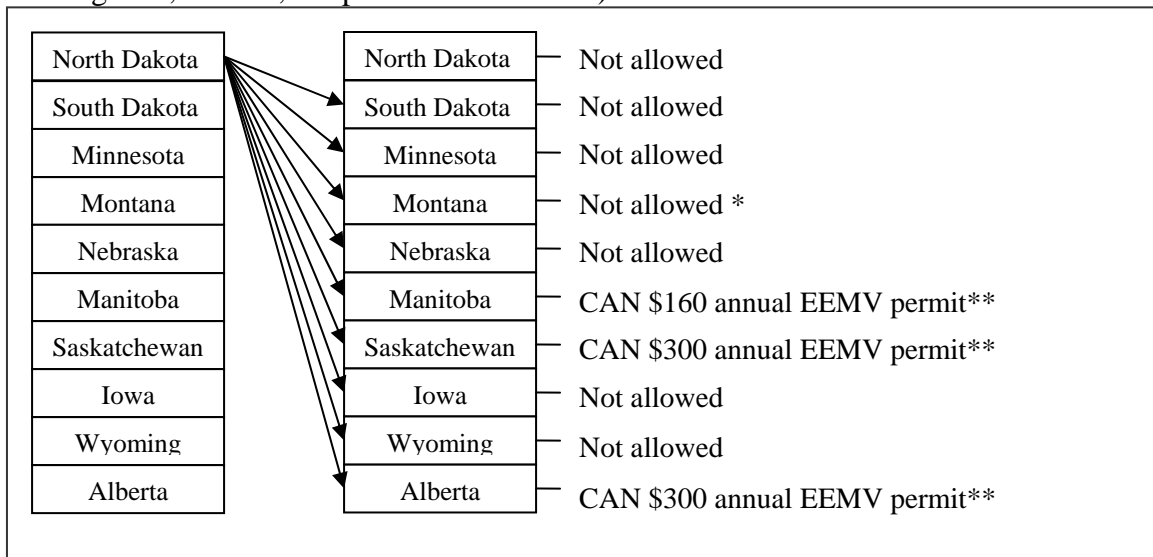
Figure 45. Scenario for a Turnpike Double (9 axles, 132,000 pounds, 12,000 pound steering axle, four 30,000 pound tandem axles).
