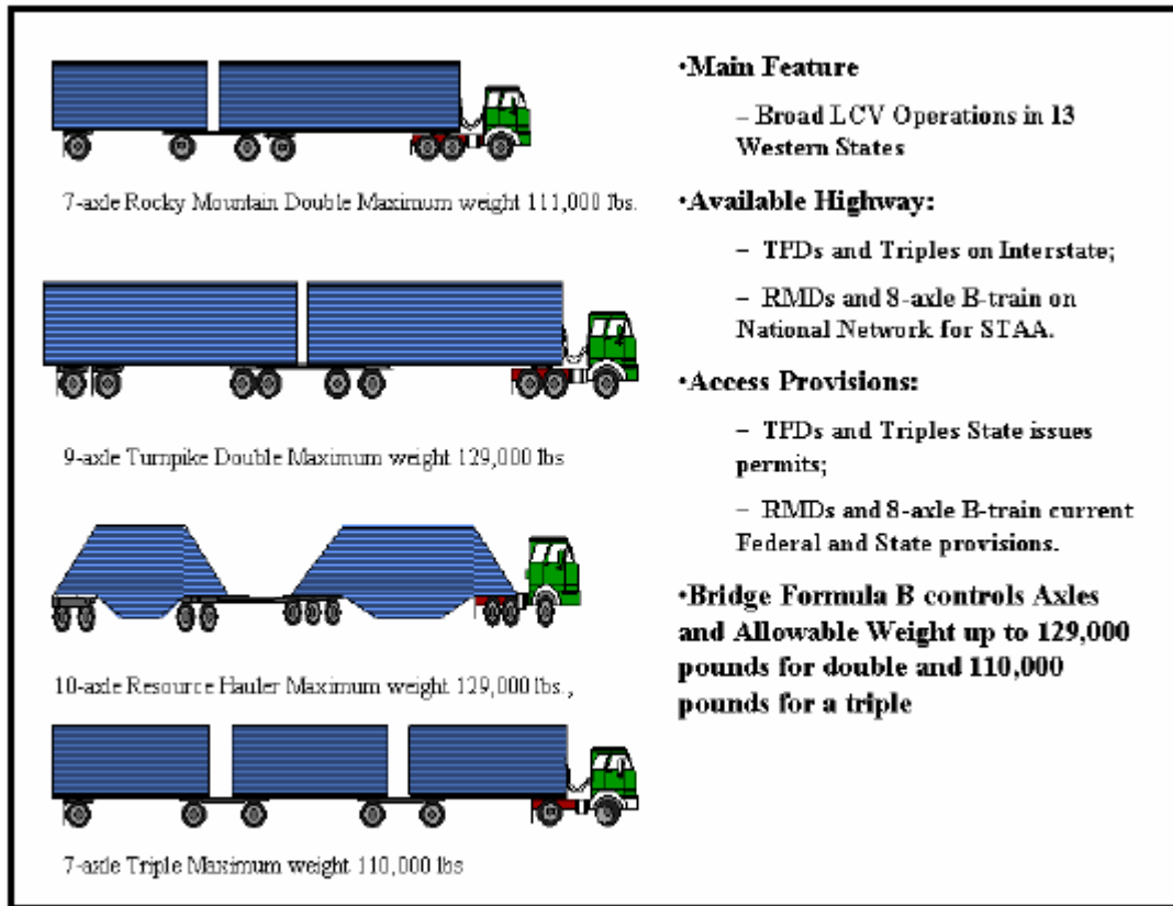
Figure 16. The Western Uniformity Scenario LCV Combinations.
